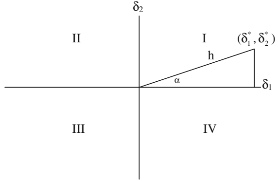
Fig. 2.2 \delta_1 and \delta_2 and the four quadrants in a two-dimensional space
