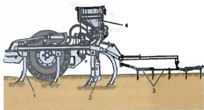
14- rasm. Sixli borona tirkalgan kultivator: 1 – yumshatuvchi organ; 2 – o'g'it solgich; 3 – sixli borona; 4 – o'g'it qutisi.
