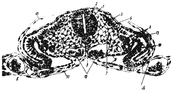
76-rasm. Tovuuq embrionidu o'q organlarining paydo bo'lishi. 1-nerv naychasi; 2-ganglioz plastinka; 3-xorda; 4-endoteliy; 5-somitlar; 6-muskul; 7-mezoderma; 8-nefrotom; 9-splanxnotom visseral varag'i; 10-pariyetal varag'i; 11-ichak endodermasi; 12-qon hujayralari; 13-ektoderma
