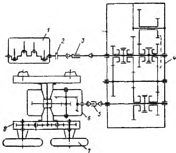
4.20-rasm. D3-99-1-4 avtogreyderi transmissiyasining kinematik sxemasi:
