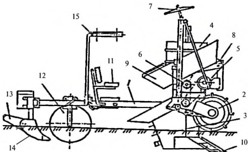
2.19-rasm. Ko'chat o'tqazadigan mashinaning tuzilishi:
