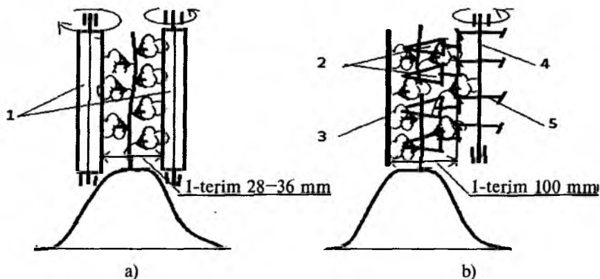
2.29-rasm. Paxtani tik (a) va gorizontal (b) shpindelli terish apparati bilan terib olish jarayonlari:
