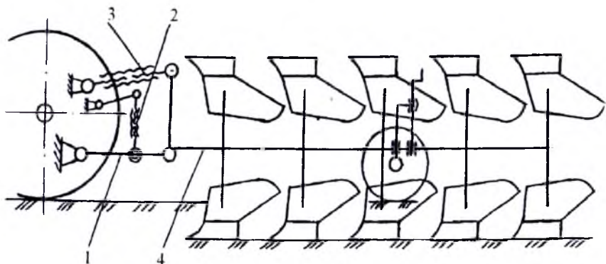
2.5-rasm. Osmo plug ramasini dala yuzasiga nisbatan paralleligini rostlash: 1 – traktor o'rnatish qurilmasining pastki tortqisi; 2 – pastki tortqining kashagi; 3 – markaziy tortqi; 4 – plug.
