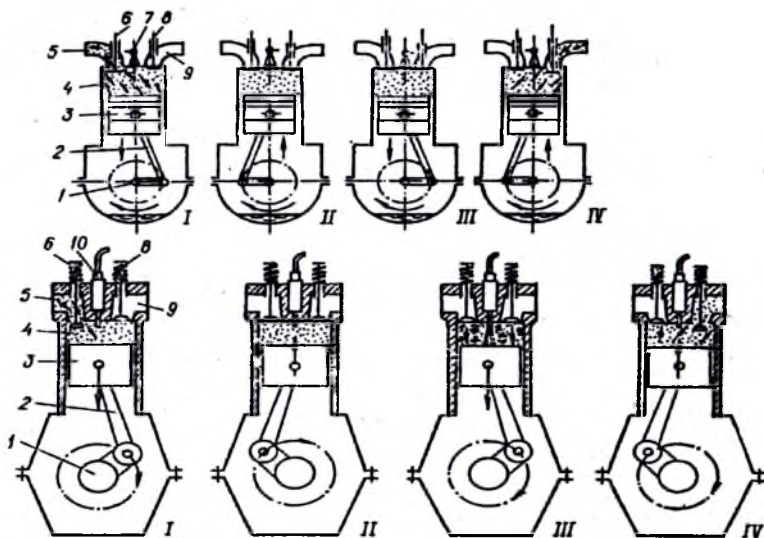
1.6-rasm. To'rt taktli karbyuratorli (a) va dizel dvigatellarning (b) ishlash sxemasi: 1 – tirsakli val; 2 – shatun; 3 – porshen; 4 – silindr; 5 – kiritish truboprovodi; 6 – kiritish klapani; 7 – o't oldirish svechasi; 8 – chiqarish klapani; 9 – chiqarish turboprovodi; 10 – forsunka; I – kiritish; II – siqish; III – kengayish; IV – chiqarish.
