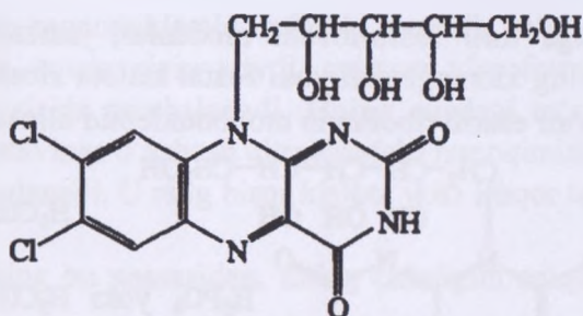
6,7-dixlor-9-ribitilizoalloksazin
