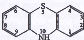
fenotiazin
