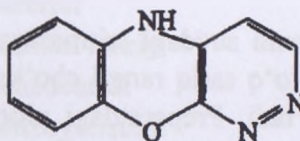
diazafenoksazin
