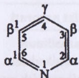
piridin
