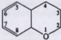
Xroman
