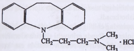
Imizin Imizinum
