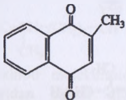
2-metil-1,4-naftoxinon (menadion)
