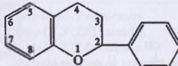
2-fenilxroman (flavan)
