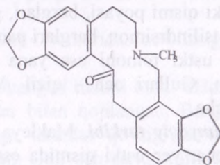
Protopin
