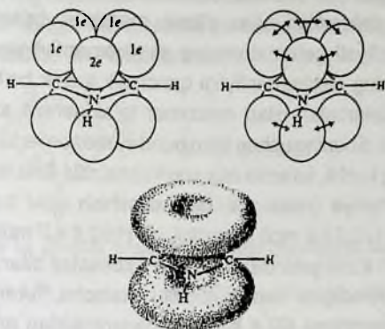
4-rasm. Pirrolning tuzilishi.
