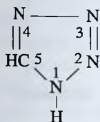
tetrazol
