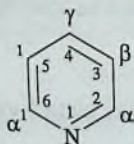
piridin
