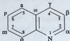
xinolin
