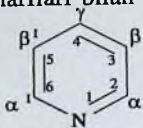
piridin
