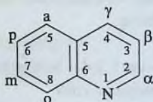
xinolin
