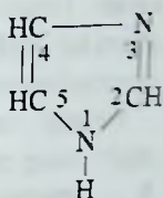
imidazol (1,3-diazol)
