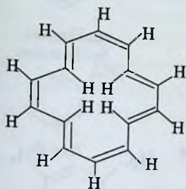
[14] – annulen
