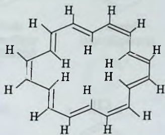
[18] – annulen
