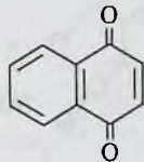
1,4-naftoxinon
