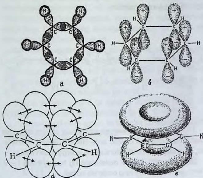
3-rasm. Benzol molekulasining tuzilishi.
