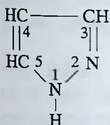
pirazol (1,2-diazol)
