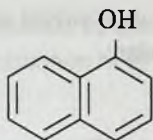
\alpha - naftol
