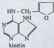
kinetin
