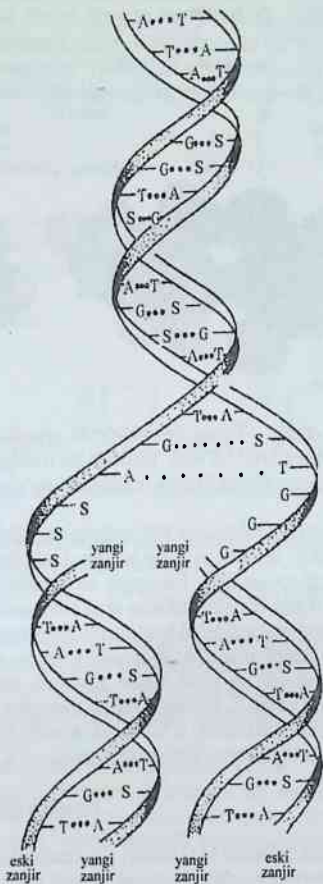
47-rasm. DNK molekulasining replikatsiyasining mexanizmi.
