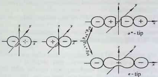
25-rasm. \sigma -bog'ning hosil bo'lishi.
