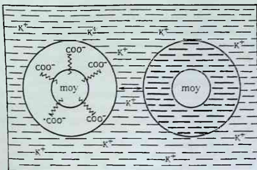
36-rasm. Suv-moy emulsiyasining detergent ta'sirida barqarorlashuvi.
