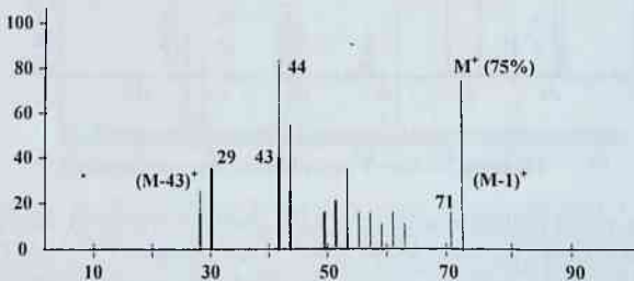
15-rasm. Moy aldegidining mass-spektri.
