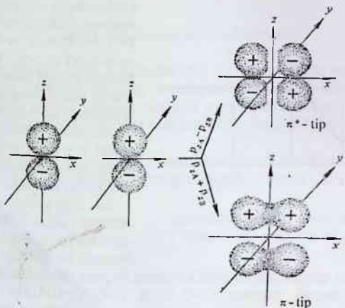
26-rasm. \pi -bog'ning hosil bo'lishi.
