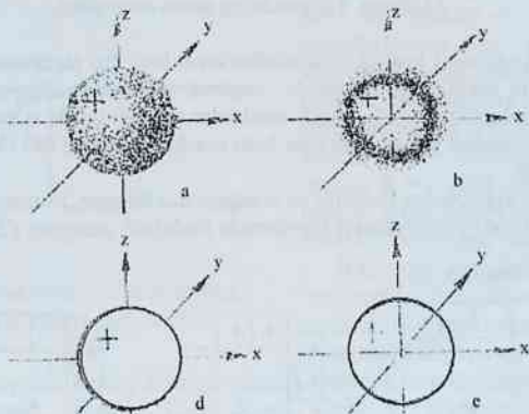
21-rasm. s-orbitallarining turlicha tasvirlanishi.
