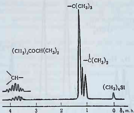
12-rasm. Izopropiluchlamchibutil oddiy efrining PMR spektri.
