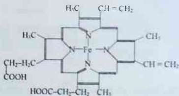
41-rasm. Gemoglobin molekulasining tuzilishi.
