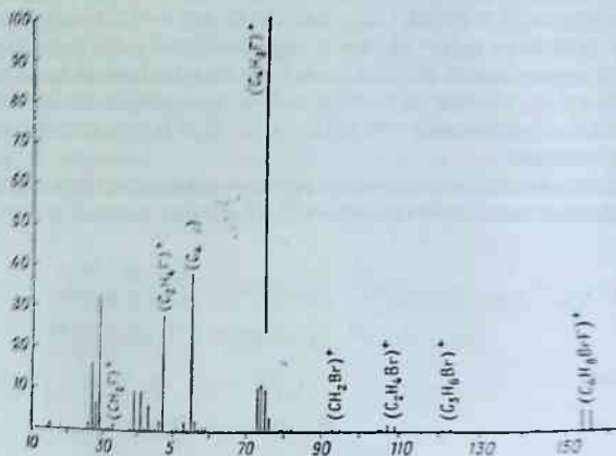
16-rasm. 1-itor-3-brombutanning mass-spektri.
