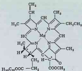
42-rasm. Xlorofill molekulasining tuzilishi.
