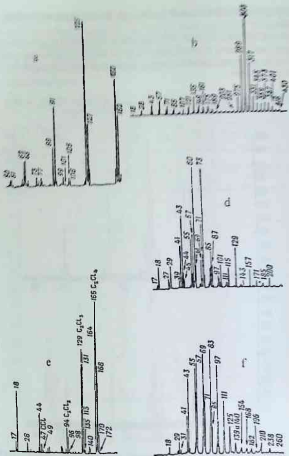
18-rasm. Dixelortoluol – (a), 2,4-di(1-etil-2,4,6-trimetilgeptil)-fenol – (b), laurin [\text{CH}_2(\text{CH}_2)_{10}\text{COOH}] kislota – (d), qizil bo'yoq tarkibidagi gaz – (c) va geptadetsil spirt – (f) larning katta tezlikda olingan mass-spektrlari.
