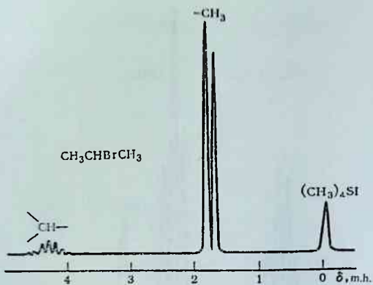
13-rasm. 2-brompropaning PMR spektri
