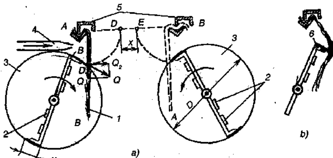
30-rasm. Xom zig'irni savash chizmasi
