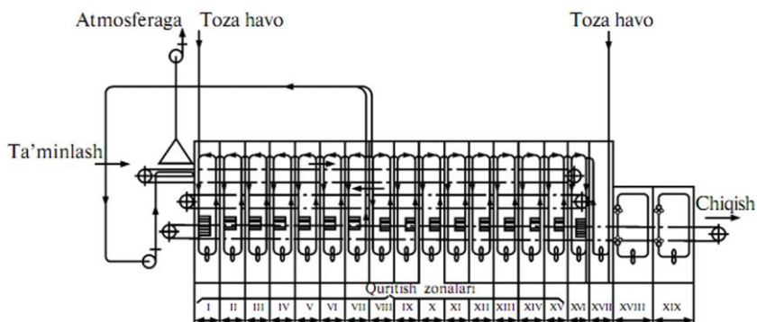
25-rasm. CKII-9-7JIM quritish mashinasining sxemasi
