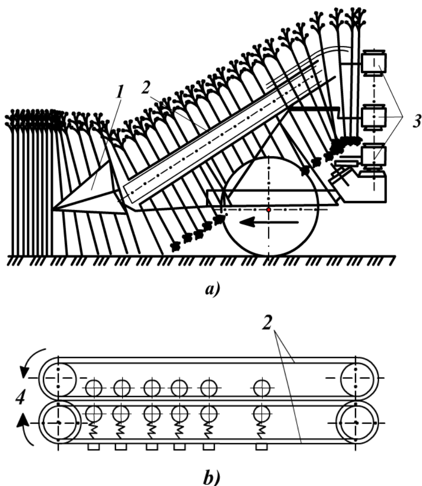
20-rasm. Zig'irpoyani yanchish mashinasining chizmasi.
