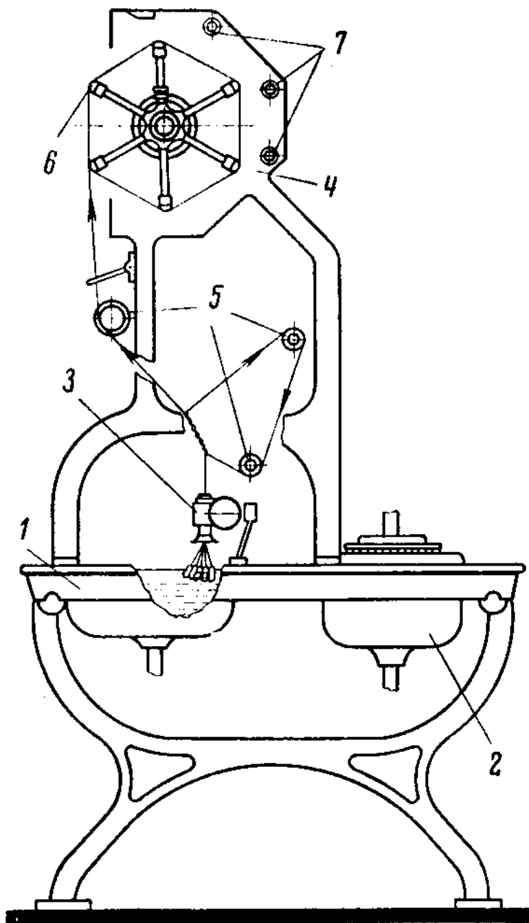
56-rasm. KMS-10VU mexanik pilla chuvish dastgohi.
