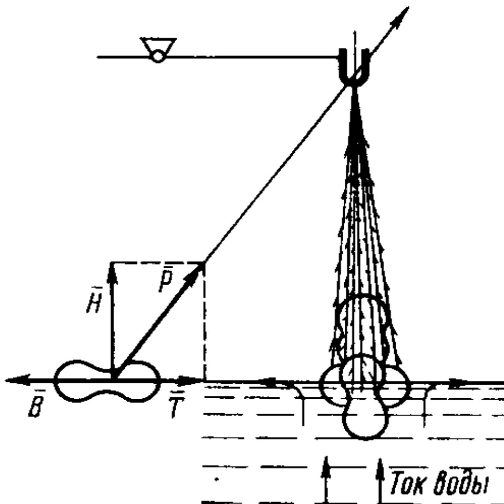
53-rasm. Silkitish jarayonida pillaga ta'sir etuvchi kuch sxemasi.
