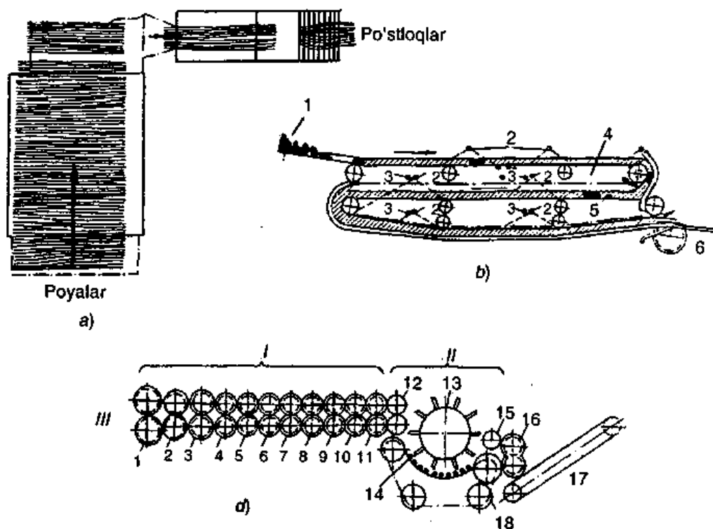
18-rasm. MT-100-K agregatining va namlash moslamasining chizmasi.
