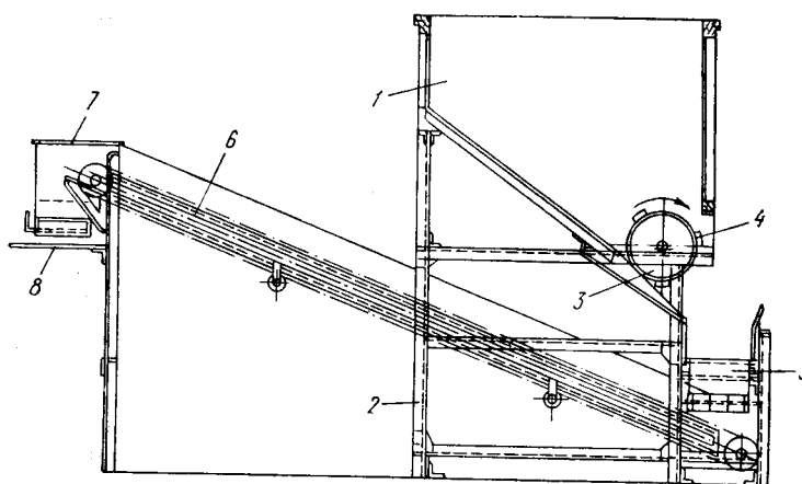
3.1.rasm. UzNIIShP sistemasidagi pilla aralashtirish dastgohi: 1- bunker, 2-rama, 3-ta'taminlash barabani, 4-planka, 5- aralashtiruvchi konveyer, 6- tushiruvchi konveyer, 7- tushirish bunkeri, 8-qopni
