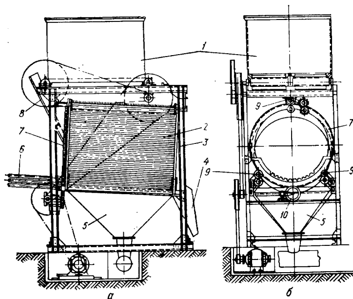
3.2.rasm. UzNIIShP sistemasidagi los tozalagich. a) yon tomondan ko'rinishi. b) old tarafdin ko'rinishi. 1-bunker, 2-baraban, 3-orqa aylana, 4-ta'minlash lotogo, 5-chang yig'ish bunkeri, 6-los ajratgich valiklar, 7-tushirish lotogo, 8-lotok, 9-rolik, 10-yuritmaning tishli aylanasi.
