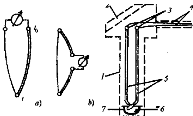
5.11-rasm. Termoelektrik o'zgartirgich:
