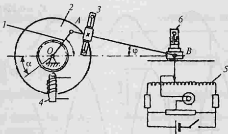
VIII.9- shakl. Burchak tezlanish datchigini tarirovkalash:
