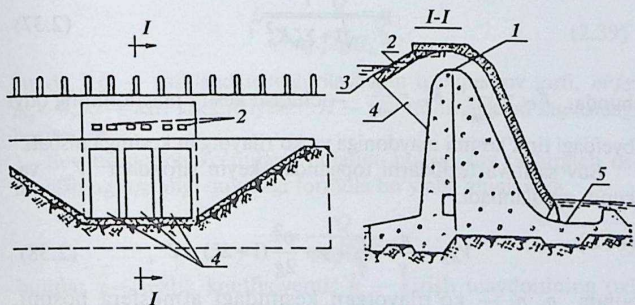
2.8- rasm. Sifonli suv tashlagich:
