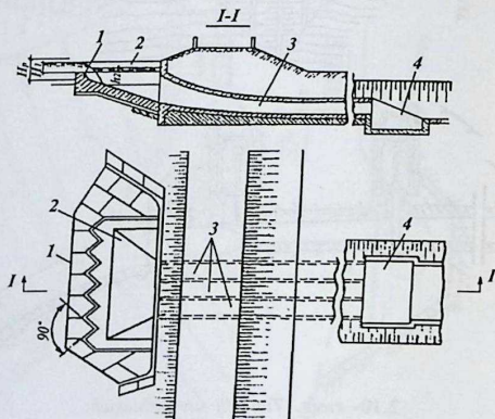
2.11- rasm. Cho'michsimon suv tashlagich:
