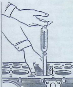
55-rasm. Porshen va silindr orasidagi tirgishni tekshirish shakli
