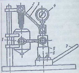
72-rasm. Forsunkalarni tekshirish asbobi
