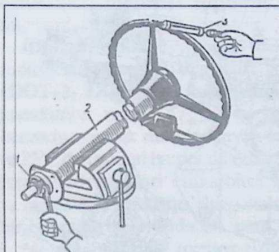
81-rasm. «ZIL-130» avtomobilining rul vali podshipnigini sozlash:
