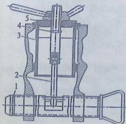
55-rasm. Porshen va silindr orasidagi tirgishni tekshirish shakli
