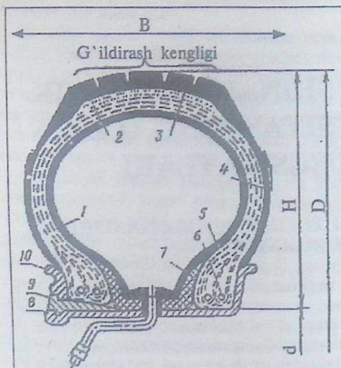
97-rasm. Yuk avtomobili kamerali shinasini to'g'in bilan yig'masining qirg'imi:
