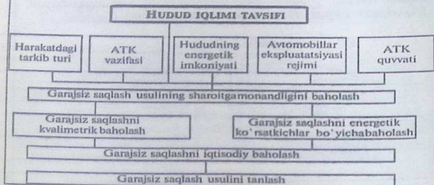
135-rasm. Garaqsiz saqlash usulini tanlash shakli
