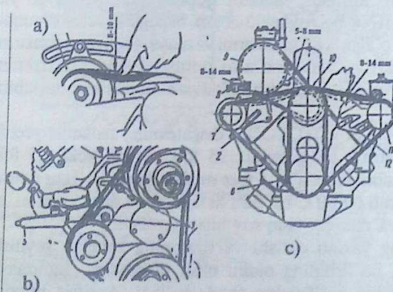
77-rasm. Dvigatellardagi yuritma moslamalarining tarangligini rostlash.
