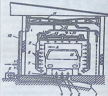
25-rasm. Harakatlanuvchi portalli avtomobillarini yuvish jihozi:
