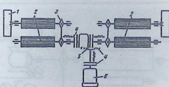
32-rasm. Rolikli inersion tormoz jihozlarning shakli:
