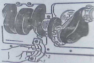
60-rasm. O'tak podshipniklarining diametral tirishini tekshirish:
