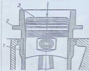
59-rasm. Porshen yig'masini silindrga o'rnatish:
