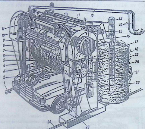
26-rasm. Yengil avtomobillar uchun harakatlanuvchi cho'tkali yuvish jihozi:
