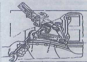
80-rasm. «ZIL-130» avtomobilidagi mexanik yuritmalilashma tepkiining erkin yo'lini rostlash
