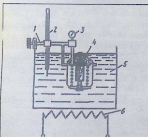
2.25-rasm. Termostatni tekshirish chizmasi
