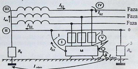
12.3-rasm. Nollash chizmasini ishlashi:
