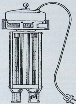
5.3-rasm. Assman aspiratsion psixrometri
