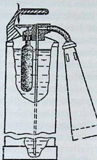
13.2-rasm. OVP - 10; havo ko'pikli o't o'chirgich
