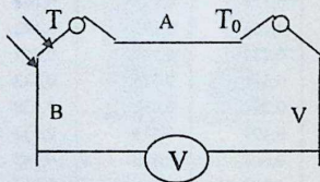
5.6-rasm. Termopara, A va V materiallardan iborat.
