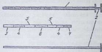
23- rasm. Murtakni ko'chirish uchun kateter: 1- temirdan tayyorlangan naycha; 2- stilet; 3- polipropyelin naycha; 4- muhit; 5- havo; 6- murtak bor muhit; 7- filtr.
