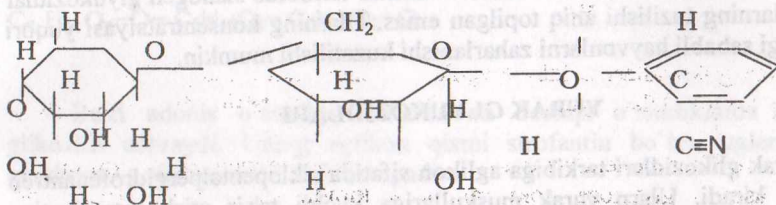
Amidalin
