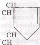
O furan
