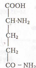
glutamin
