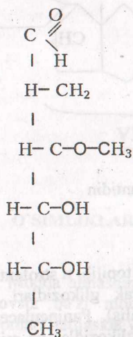
simoroza
