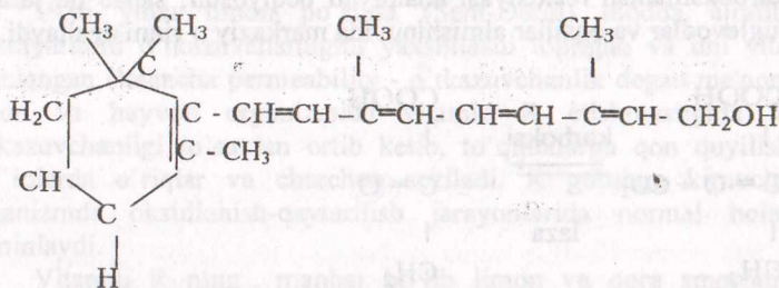
Vitamin A 2
