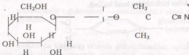
Linamarin
