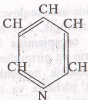
Piridin
