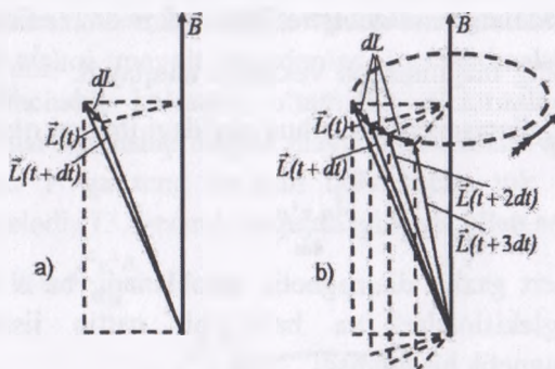
13.8-rasm. Elektronning orbita bo'ylab harakati
