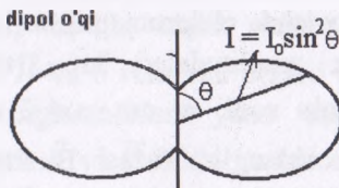
15.2- rasm. Elementar dipolning nurlanishini
