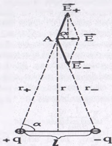
1.3-rasm. Kuchlanganlikni hisoblash uchun chizma
