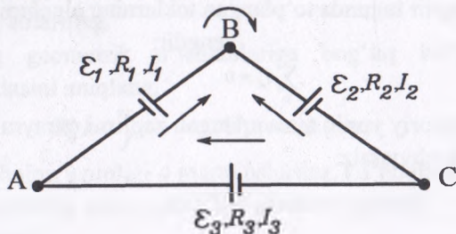
5.12-rasm. To'la zanjir ko'rinishi
