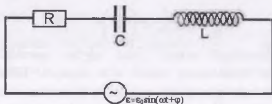
14.7-rasm. O'zgaruvchan tok zanjiri
