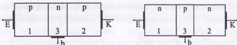
8.20-rasm. Yarimo'tkazgichli triod (transistor)
