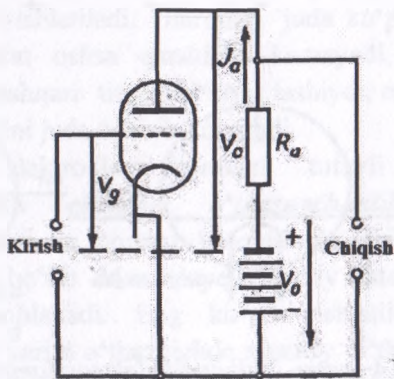
8.13-rasm. Triod lampali kuchaytirgich sxemasi
