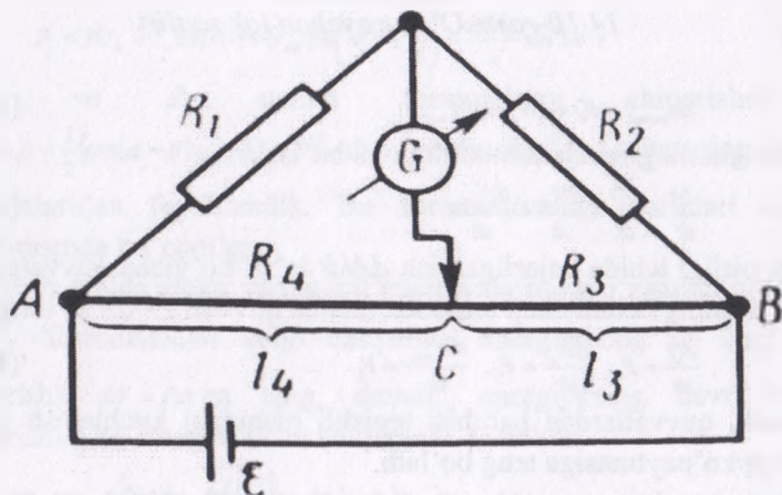
14.9 – rasm. Reaxordli Uitson ko'prigi
