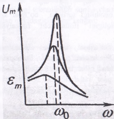
14.3 rasm. U_m ning \omega ga bog'liqlik grafigi
