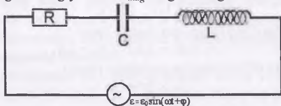
14.10-rasm. O'zgaruvchan tok zanjiri
