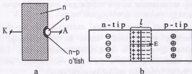
8.19- rasm. Yarim o‘tkazgichli diod
