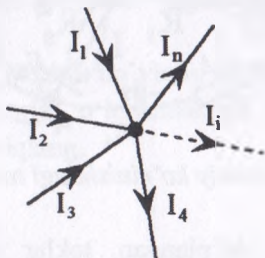
5.11-rasm. Tok zanjiridagi tugunning ko'rinishi
