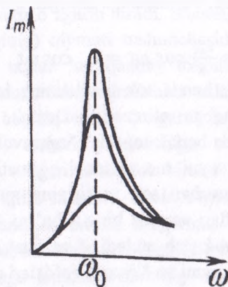
14.4-rasm. I_m ning \omega ga bog'liqligini
