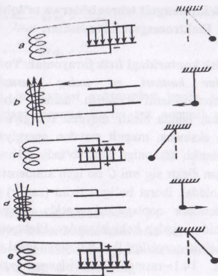
14.1-rasm. Tebranish konturida tebranishlarni hosil qilish
