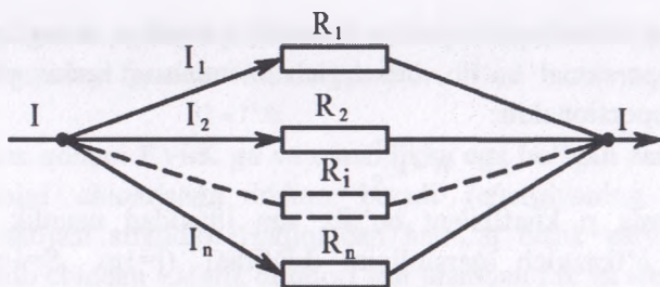
5.5-rasm. O'tkazgichlarni parallel ulash
