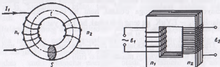
12.3-rasm. Transformatorning tuzilishi
