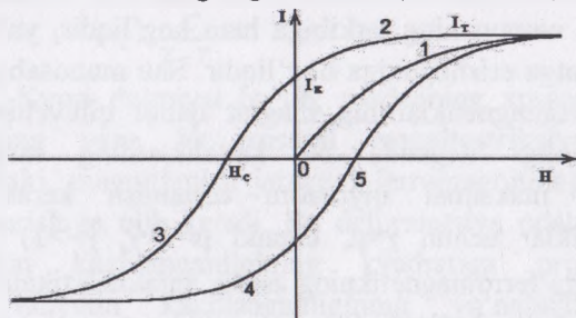
13.12-rasm. Gistrezis sirtmog'i
