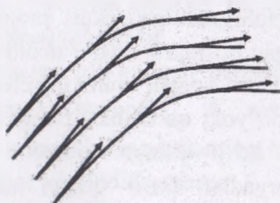
1.5-rasm. Kuch chiziqlarining chizmasi
