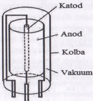
8.2-rasm. Termoelektron emissiya hodisasi
