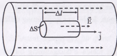
5.8-rasm. Silindrdan tok o'tishini hisoblash chizmasi
