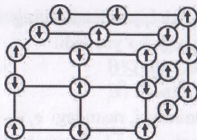
13.15-rasm. Kristall magnit panjarasi
