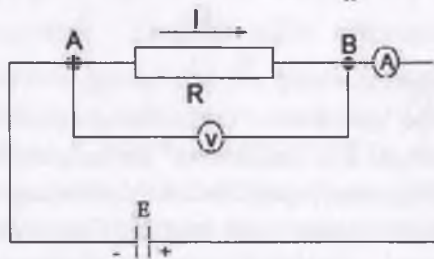
5.3-rasm. O'zgarmas tok zanjiri
