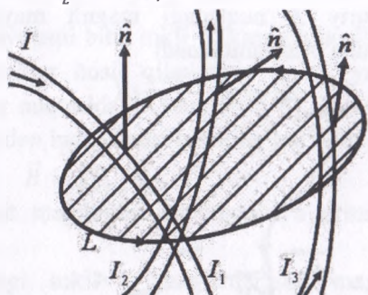
11.2-rasm. Sirkulyatsiyasini hisoblash chizmasi
