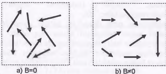
13.9-rasm. Paramagnit moddalarda qutblanish
