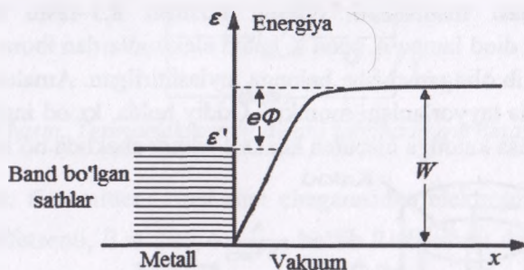
8.1-rasm. Fermi sathi energiyasi
