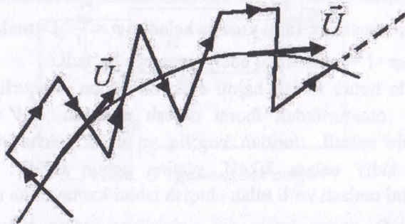
5.2-rasm. Zaryadlangan zarrachalarning harakat traektoriyasi
