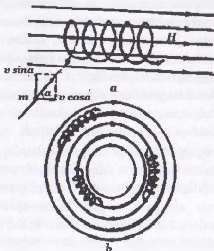
10.3-rasm. Zaryadning spiral simon harakati
