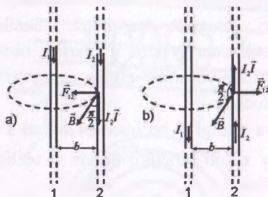
10.1-rasm. Parallel tokli o'tkazgichlarning o'zaro ta'siri
