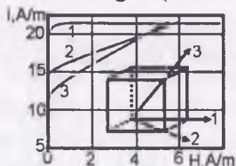
13.13-rasm. Temirning elementar panjara yacheykasi
