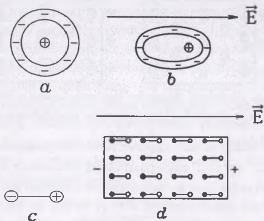
3.4-a, b, c, d rasm. Qutibsiz molekulalarning qutblanish jarayoni
