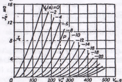
8.12-rasm. Anod tokning anod kuchlanishiga bog'liqlik grafigi
