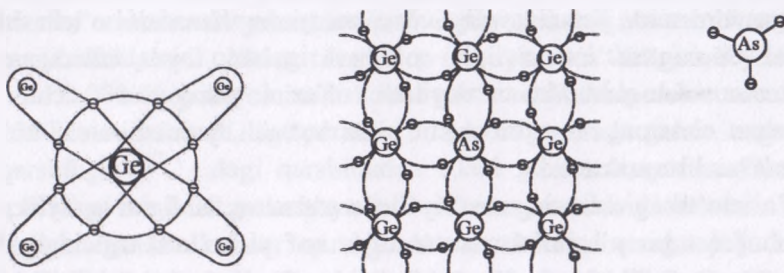
8.15-rasm. Yarimo'tkazgich tuzilishi
