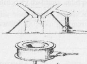
49-rasm. Issiq holda filtrlash uchun voronkalar: a-suv bilan isitish; b-elektr bilan isitish.
