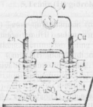
85-rasm. Galvanik element: 1- mikrostackanchalar, 2-taglik, 3-elektrolit ko'prik, 4-galvanometr.
