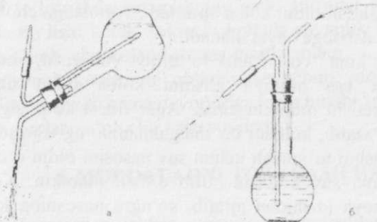
52-rasm. Yuvgichni suv oqimini olish uchun ishlatilishi: a- keng oqim, b-ingichka oqim.
