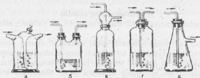
61-rasm. Yuvuchi sklyankalar: a-Tishenko sklyankalari; b-ikki bo'yinli sklyanka; v, g, d-yuvichlar.
