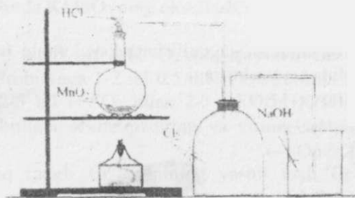
Rasm. Xlorning olinishi
