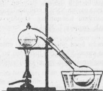
81-rasm. Nitrat kislotalari olish uchun asbob
