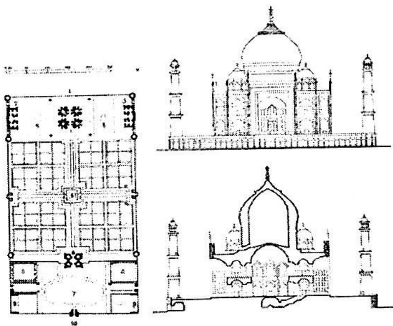
30-rasm. Tojmahal. Tarh, tarz, qirqim
