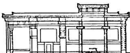
14-rasm. Megaron. Qirqim. Tarh
