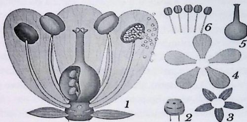
15- rasm. Gulning tuzilishi: 1 – gulning uzunasiga kesmada; 2 -gulbandi; 3 - gulkosabarglar; 4 – tojbarglar; 5 - urug'chi; 6 –changchi.
