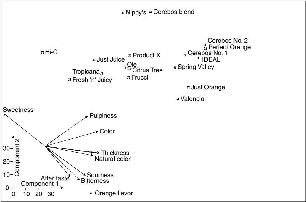
FIGURE 14.4 Results of a PCA on orange drinks showing both the relationships of the products to each other and the associations among the original descriptive attributes. The plot of the products is offset from the plot of the attributes to aid the visual presentation while maintaining the relative directions and magnitudes. For example, Hi-C is high in sweet and low in sour and bitter, whereas Cerebos No. 2 is less sweet and relatively high in pulp, color. (From H.R. Cooper, M.D. Earle, and C.M. Triggs. 1989. Product Testing with Consumers for Research Guidance , L.S. Wu, ed., Philadelphia, PA: ASTM International. With permission.)
