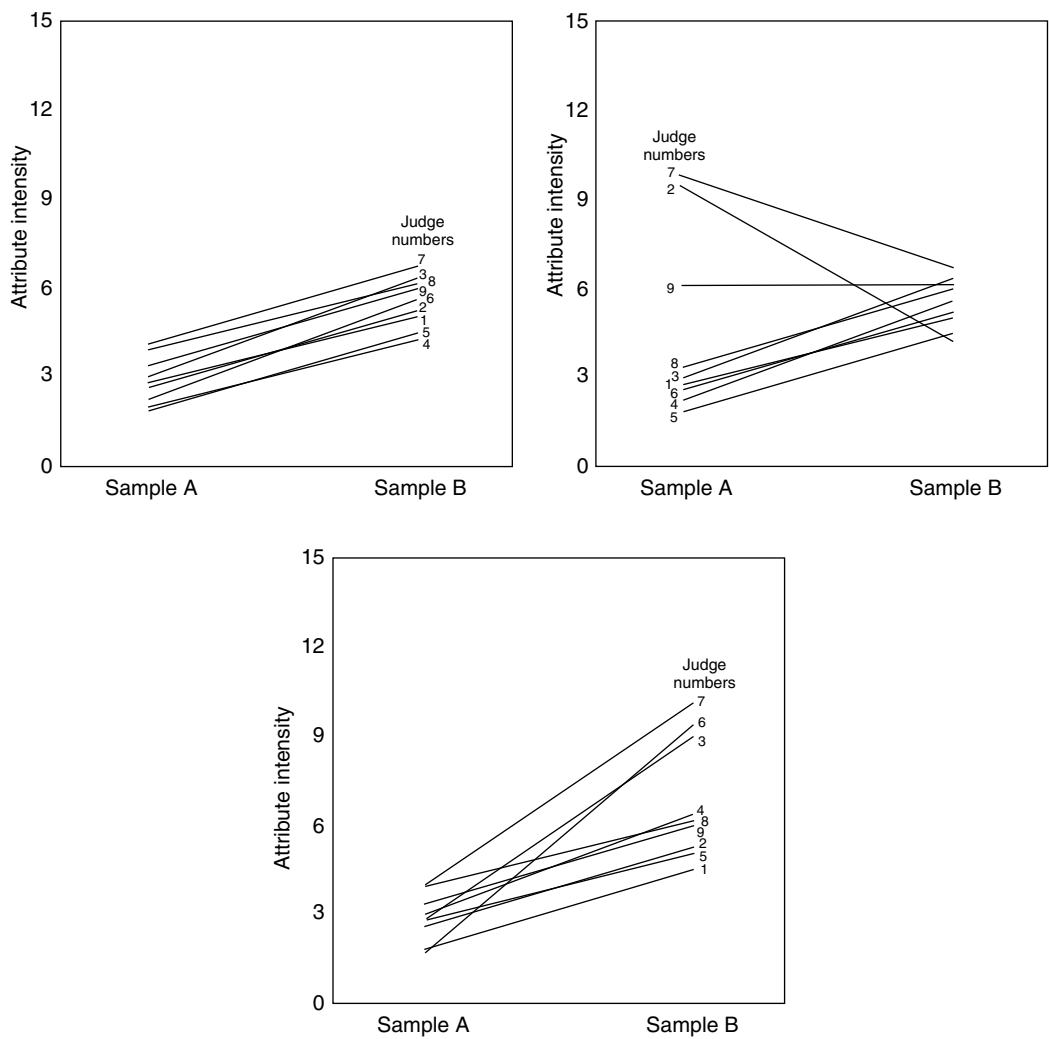
FIGURE 9.2 Judge and sample interaction plots (see text).
