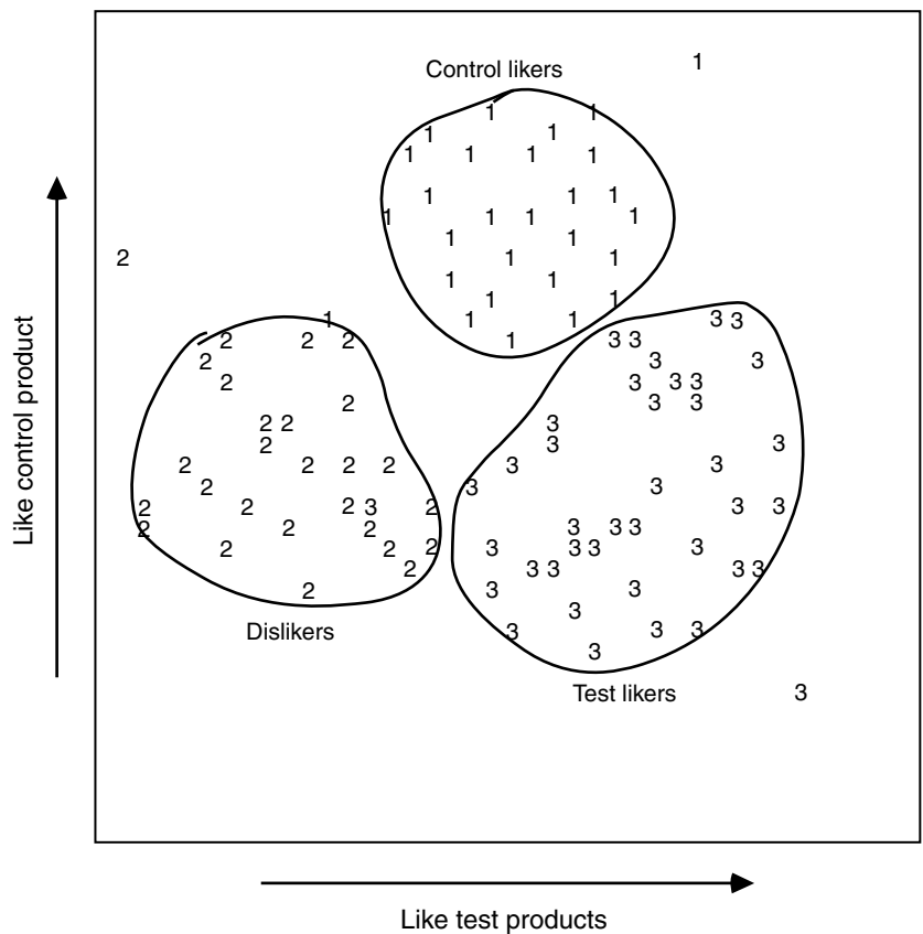
FIGURE 14.6 A plot of three clusters of respondents grouped by their patterns of overall liking for a group of yogurt products. The plot shows how the overall mean of the three groups would be a poor summary of the “average” liking for a product.
