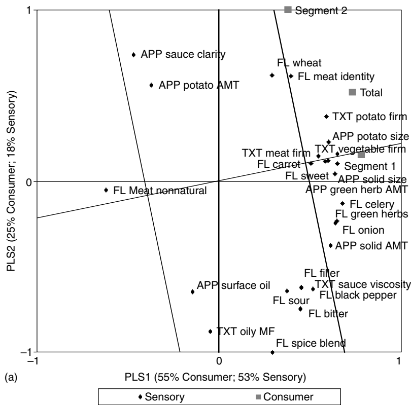
FIGURE 14.22 PLS maps illustrating positive and negative drivers by segment. Chart (a) illustrates that segment 1 prefers lots of large and firm meat, potato and vegetable pieces and high intensities of meat identity, green herb, carrots, onion and celery flavors and low intensity of nonnatural meat flavor. Chart (b) illustrates that segment 2 prefers lots of large firm potatoes in a clear, low viscosity sauce, high meat identity flavor, low oiliness, and low spiciness (especially black pepper).
