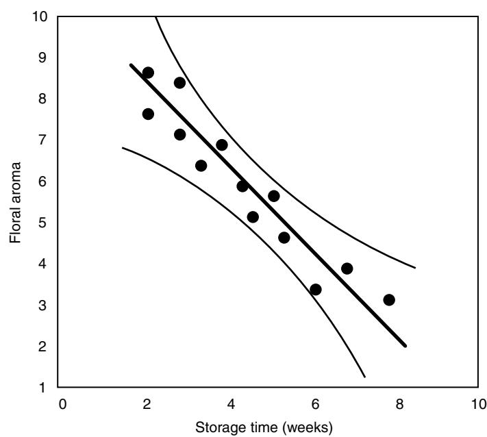
FIGURE 14.8 A fitted regression line with 95% confidence bands. The width of the bands provides a visual assessment of the quality of the fitted line. Narrow bands such as these indicate that the data are well fitted by the line, while wide bands indicate that a large amount of unexplained variability remains.
