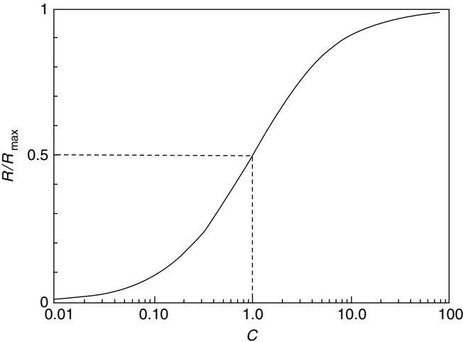
FIGURE 5.5 The sigmoidal relationship between taste response, R/R_{\max} , and stimulus concentration, C , as specified by the Beidler equation; k is set equal to 1 for convenience. The inflexion point (maximum slope) of the curve occurs at R=0.5R_{\max} when C=k .
