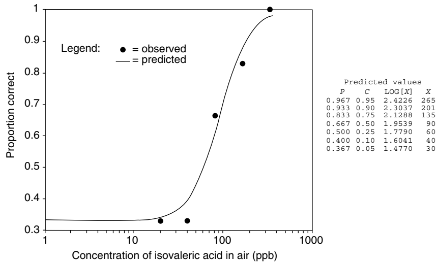
FIGURE 8.4 Fitting of a dose–response curve to the data in Table 8.2 using “SAS® PROC NLIN” and the logistic method. The estimated value of T=1.954 is the threshold concentration in log(ppb) for Panelist 13. P , proportion correct; X , concentration; P_c , proportion correct, 0.0–1.0; P_d , proportion distinguishers = % above chance.
