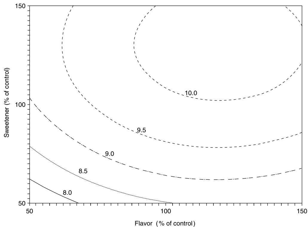
FIGURE 14.27 A contour plot of the predicted relationship between overall liking and the levels of sweetener and flavor in the product. Contour plots provide a quantitative assessment of the sensitivity of the product to changes in the levels of the ingredients.
