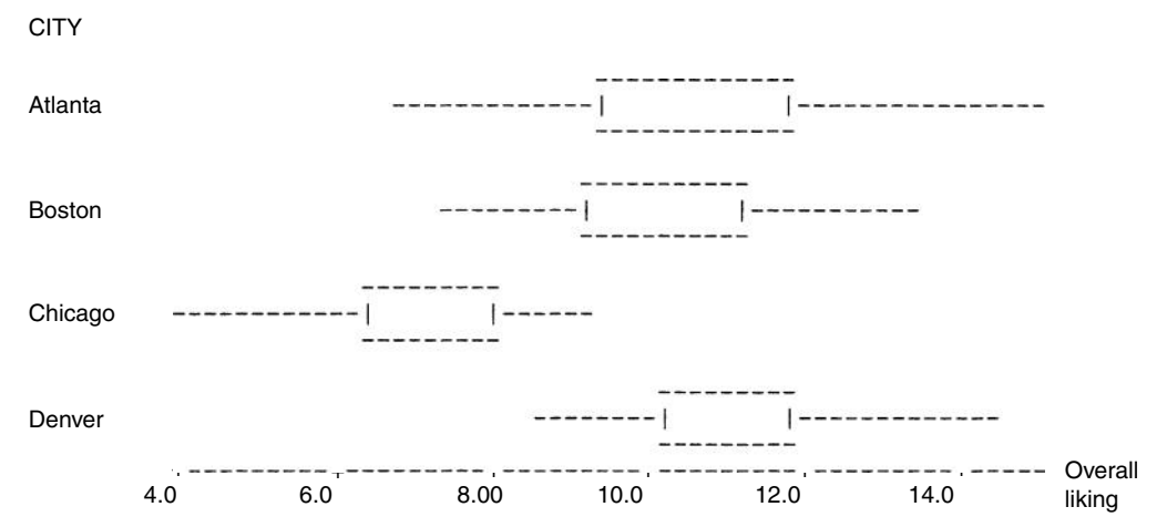
FIGURE 13.3 Box-and-whisker plots of the overall liking scores from the multicity consumer test data in Table 13.1.
