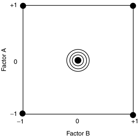
FIGURE 14.28 A two-factor, first-order RSM experiment. The figure illustrates the arrangement of the factorial and center points in an RSM experiment with two independent variables that permit estimation of a first-order regression model in Equation 14.14.
