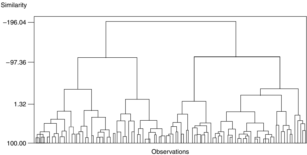
FIGURE 14.16 The dendrogram of the consumers’ centered overall liking ratings suggests either two or four segments. The two segment solution was chosen because two of the segments in the four-segment solution have fewer than 25 respondents in them.
