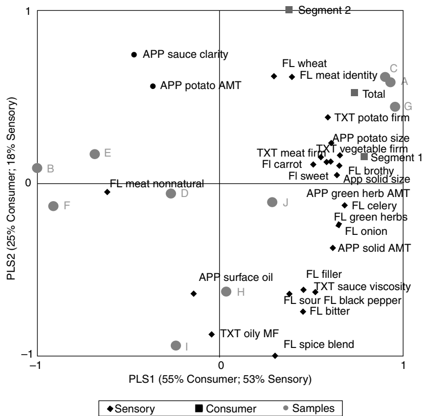
FIGURE 14.21 PLS map of prepared meals showing distribution of test products and difference between preference segments. Both segments like products A, C, and G. Segment 1 dislikes products B, E, and F. Segment 2 dislikes products H and I.
