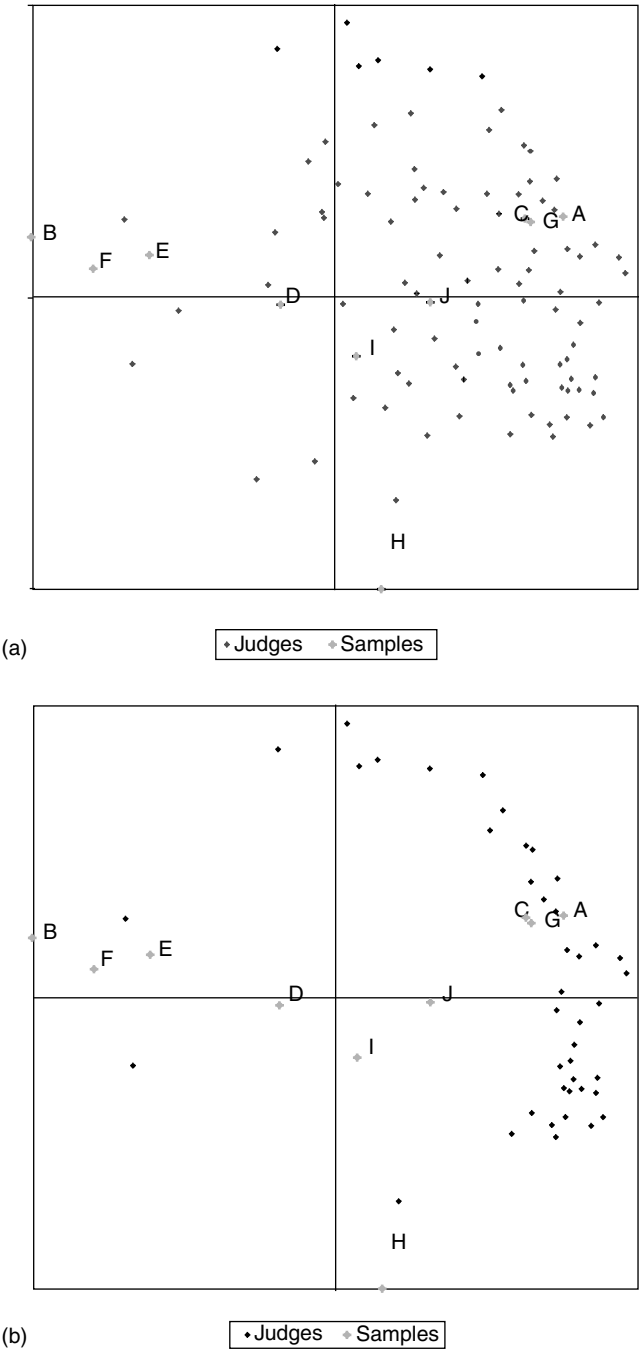
FIGURE 14.12 (a) A plot of the rescaled factor scores of the products and the factor loadings of all respondents. (b) A plot of the rescaled factor scores of the products and the factor loadings of respondents with communalities greater than 0.50—i.e., the respondents for which the model explains at least 50% of the variability in their liking ratings. (c) A plot of the rescaled factor scores of the products and the factor loadings of respondents rescaled to fall equidistant from the origin. This optional step sometimes makes it easier to identify clusters of respondents. (d) The final internal preference map including sensory attributes. The coordinates of the sensory attributes are their correlations with the factor scores of the samples from each of the two dimensions of the map.
