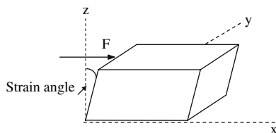
FIGURE 3.17 A solid undergoing shear deformation due to the shearing force F .
