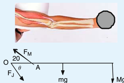
FIGURE 7.31 An outstretched arm supporting a dumbbell (above) with equivalent forces drawn for analysis (below).
