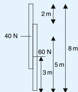
FIGURE 7.30 Ladder dimensions.
