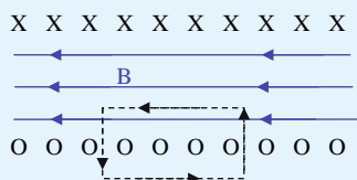
FIGURE 17.23 (left) A solenoid made from winding wire around a metal core; (right) a longitudinal cross-section of the center portion of a solenoid showing the cut windings with current flowing around from the bottom to the top (counterclockwise, as viewed from the left), producing a uniform B field to the left. The rectangular Amperian loop is used to evaluate Ampere's law in order to find the B field inside the solenoid.
