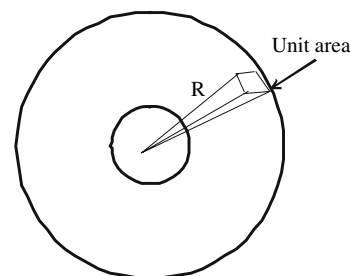
FIGURE 11.4 The power radiated from a point source into the pyramid shown with vertex at the source is a constant, thus the power density, or intensity, must decrease according to Equation (11.4).
