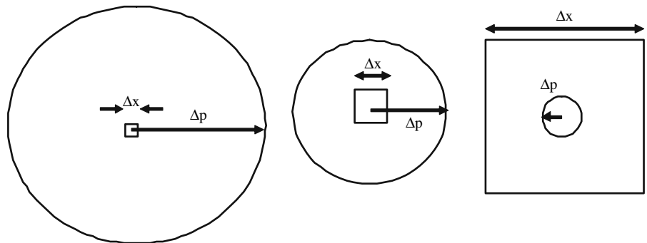
FIGURE 24.9 The uncertainty in the x -location of a particle is inversely related to the uncertainty in its momentum along the x -direction. The product of these two uncertainties must be at least the order of h = 6.63 \times 10^{-34} J-s.
