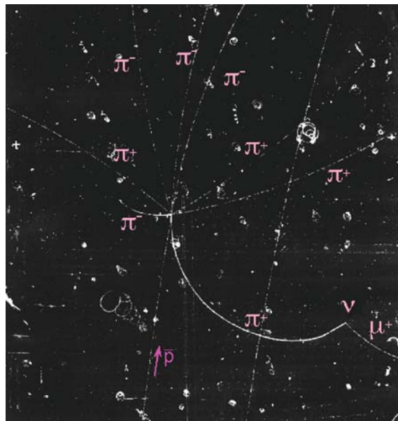
FIGURE 14.3 Bubble chamber photo of the trail of an antiproton (labeled as \bar{p} ) colliding with a stationary proton, annihilating each other to create pure energy which in turn created 8 pions ( \pi ). The chamber lies in a strong magnetic field that curves the oppositely charged particles in opposite directions. One of the pions subsequently decays into a muon and a neutrino which leaves no track.
