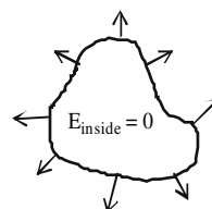
FIGURE 14.16 A metal object with a net charge that distributes itself on the surface producing an external E field perpendicular to the surface but having zero internal E field.
