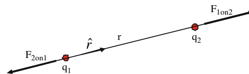
FIGURE 14.4 The pair of equal and opposite Coulomb's law forces between two like point charges.
