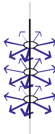
FIGURE 14.15 By symmetry, the electric field from a long charged wire must be radially directed and depend only on the distance from the wire (away from the ends of the wire).
