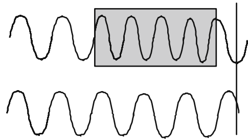
FIGURE 22.2 Two initially in-phase light waves traveling to the right, showing the optical path difference when one wave passes through a different optical medium with a larger index of refraction
