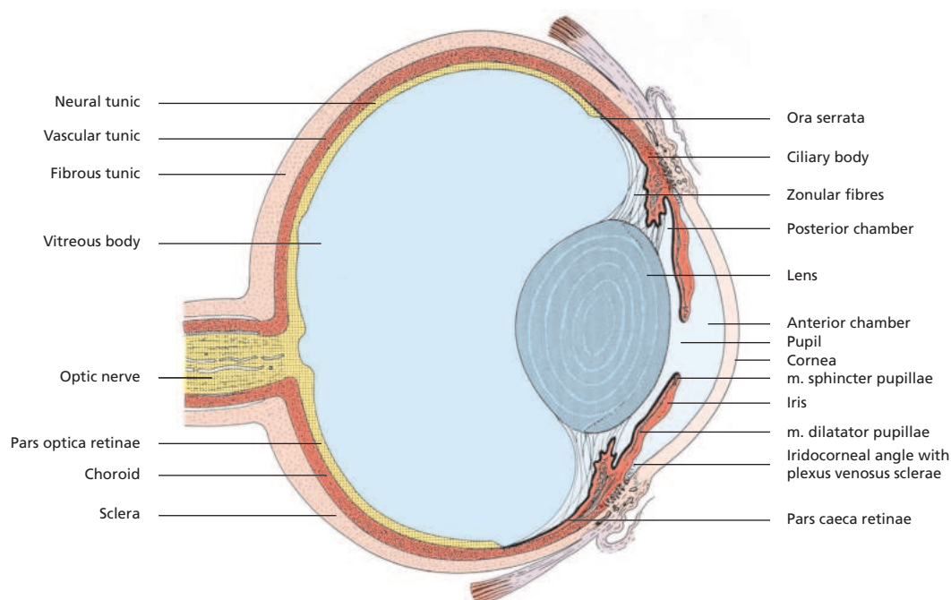
16.11 Bulb (schematic).
