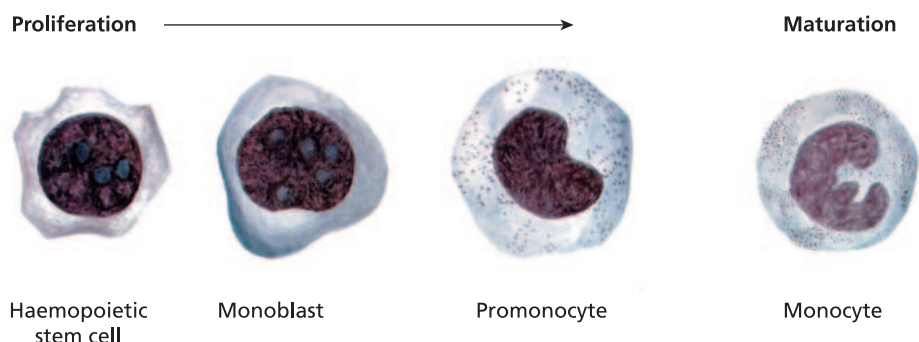
7.12 Monocytopoiesis (schematic).
