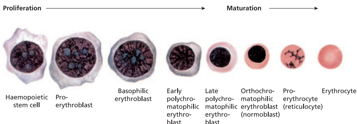
7.2 Erythropoiesis (schematic).
