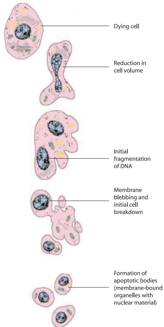
1.41 Apoptosis (schematic).
