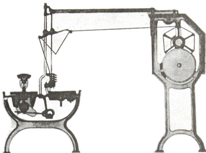
35-rasm. Oilalardan yakka tartibda tanlab olingan pillalarni tirik holida chuvatilib, ipini olishga mo'ljallangan moslama.
