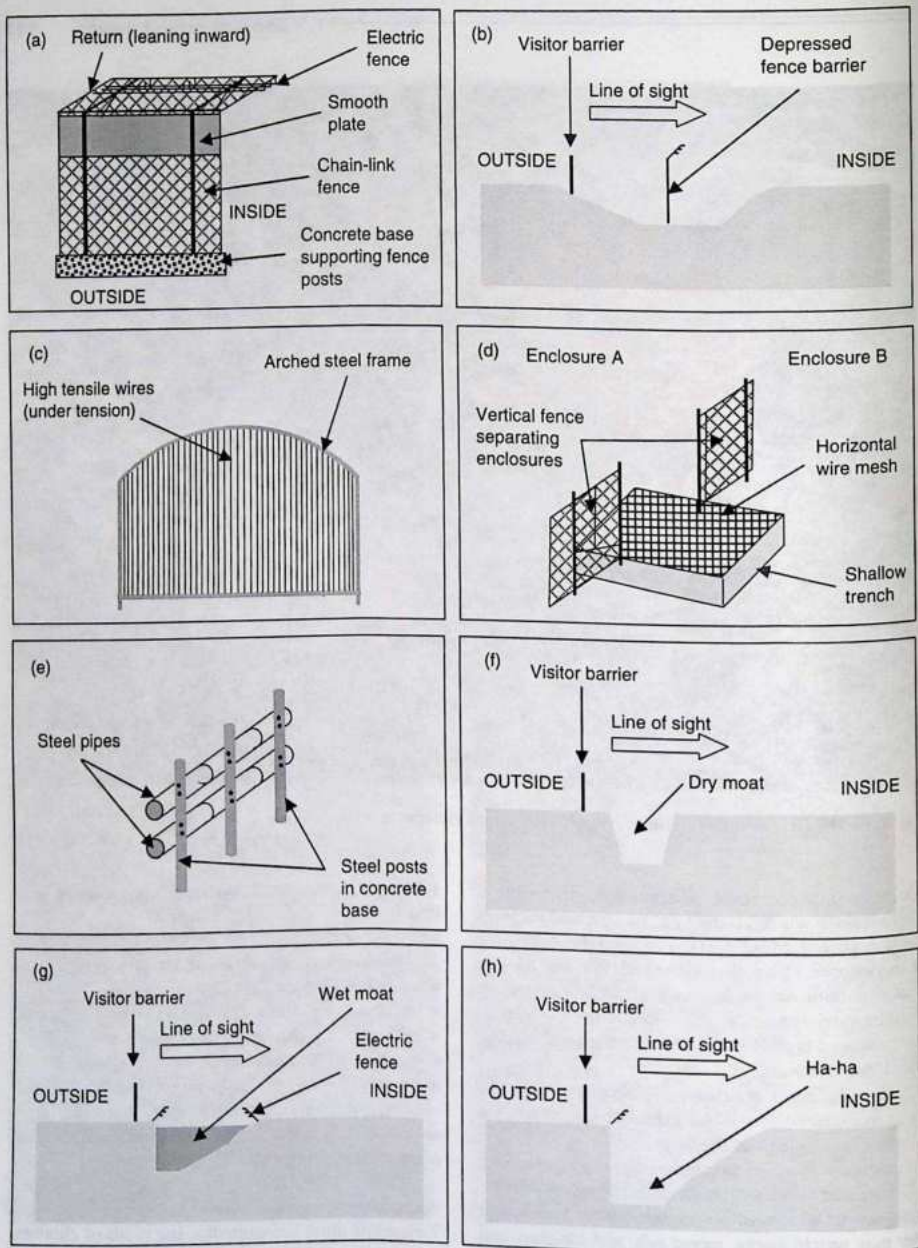
Fig. 7.20 Some common barriers found in zoos: (a) chain-link fence with return; (b) depressed fence; (c) high tensile vertical wire fence; (d) horizontal wire fence between adjacent enclosures; (e) reinforced pipe barrier; (f) dry moat; (g) wet moat; (h) ha-ha.
