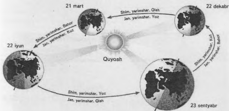
16-rasm. Yerning quyosh atrofidan aylanishi
