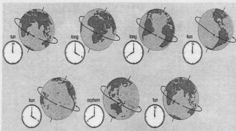
15-rasm. Yerning o'z o'qi atrofida sutkalik aylanishi
