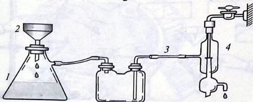
14-rasm. Past bosimda filtrlash.
