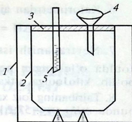
25-rasm. Kalorimetr:
