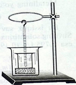
23-rasm. Soddalashtirilgan kalorimetr.
