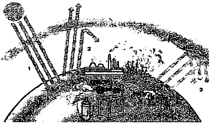
8.3-rasm. “Issiqxona samarasi” hodisasi
