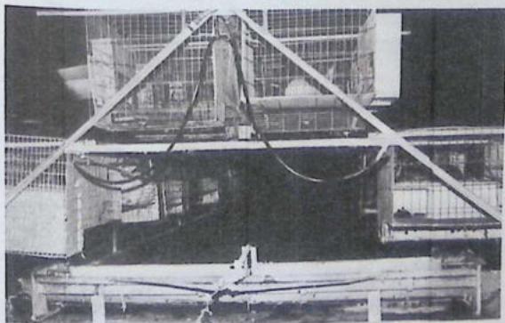
Fig. 4.11. A two-tier caging arrangement with an automatic manure scraper powered by a small electric motor. (Courtesy of OSU Rabbit Research Center)
