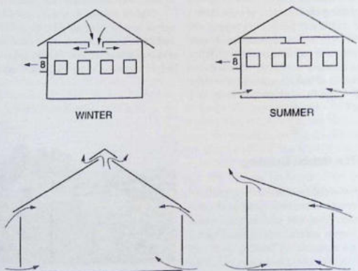
Fig. 4.2. Placement of winter and summer air inlets and outlets for a mechanically ventilated rabbit building (top) and for naturally ventilated buildings (bottom). (Courtesy of James A. Moore)
