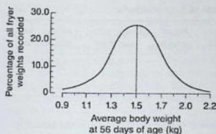
Fig. 15.5. Bell-shaped curve or normal distribution characterizing a quantitative trait. (Courtesy of S.D. Lukefahr)
