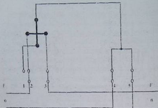
11.3-rasm. CTK1 hisoblagichlarining ulanish sxemasi
