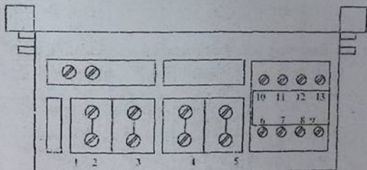
11.2-rasm. CTK1 hisoblagich klemmlarining joylashishi
