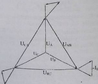
8.3-rasm. Kuchlanishning simmetriklik holati.
