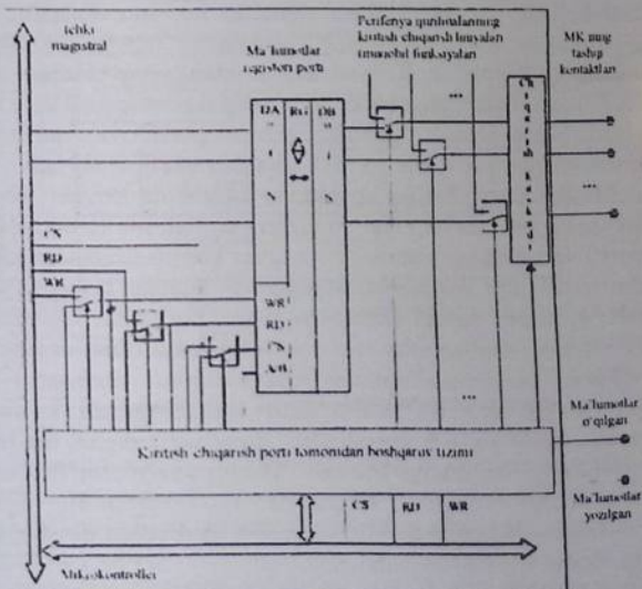
4.8-chizma. Kiritish chiqarishning parallel porti tuzilmasi
