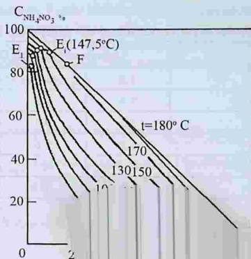
4.1- rasm. \text{NH}_4\text{H}_2\text{PO}_4 diagrammasi (F – ev)
