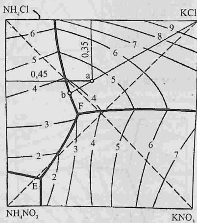
2.5- rasm. KCl – NH_4NO_3 – KNO_3 – NH_4Cl sistema izotermasi (40°C).
