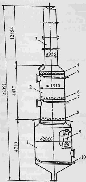
5.14- rasm. Qo'shimcha neytrallagich:
