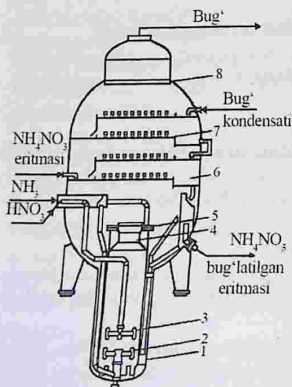
4.8- rasm. Nitrat kislotani neytrallagich (NIF):
