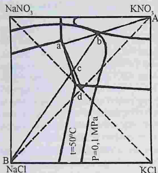
2.2- rasm. Izotermik ( 50^{\circ}\text{C} va izobarik ( 0,1\text{ MPa} ) kesishuvli diagrammada \text{KCl} + \text{NaNO}_3 = \text{NaCl} + \text{KNO}_3 konversiyaning optimal sikli.
