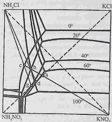
2.8- rasm. \text{KCl} - \text{NH}_4\text{NO}_3 - \text{KNO}_3 - \text{NH}_4\text{Cl} sistema politermasi.
