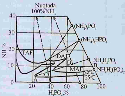
3.1- rasm. 25 va 75°C haroratdagi \text{NH}_3 - \text{H}_3\text{PO}_4 - \text{H}_2\text{O} sistemadagi eruvchanlik izotermsi.
