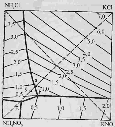
2.7-rasm. KCl – NH 4 NO 3 – KNO 3 – NH 4 Cl sistema izoterma (100°C).
