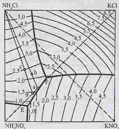
2.6- rasm. KCl – \text{NH}_4\text{NO}_3 – \text{KNO}_3 – \text{NH}_4\text{Cl} sistema izotermasi ( 60^\circ\text{C} ).
