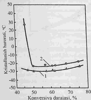
5.1- rasm. SKO' kristallanish haroratining P_2O_5 konversiya darajasiga bog'liqligi:
