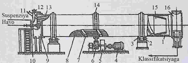
3.7- rasm. Barabanli donadorlash-quritgichi (BDQ):
