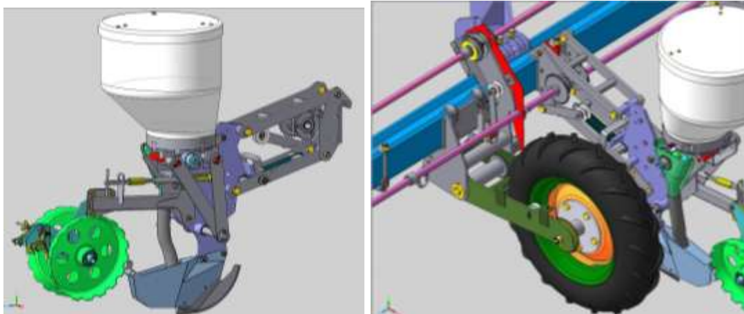
37-rasm. Chigit ekish seyalkasining mexanizmlari
