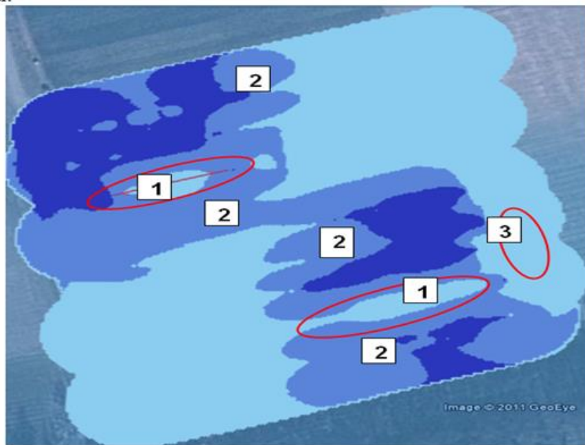
7.2-rasm. Off-line texnologiyasi uchun azot solish xaritasi
