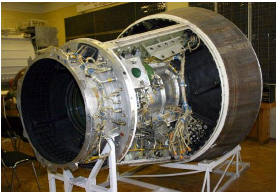
4.5-rasm. Kosmosdan turib tasvirga olish apparatining ko'rinishi
