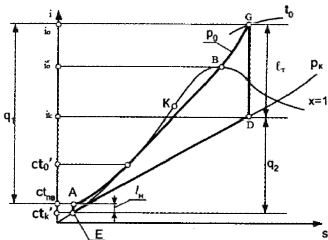
1.14-rasm. I, s - diagrammaga BKU sikli
