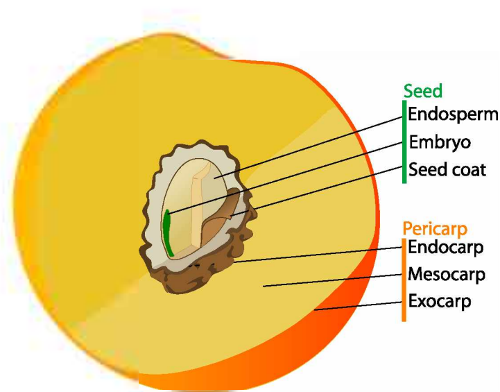
Figure 8.18. Scheme of drupe (e.g., peach) with three levels of pericarp. Note that pit is essentially endocarp + seed.
