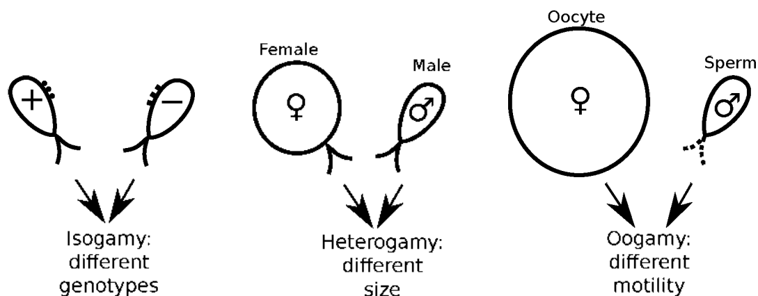
Figure 4.4. Three types of syngamy.
