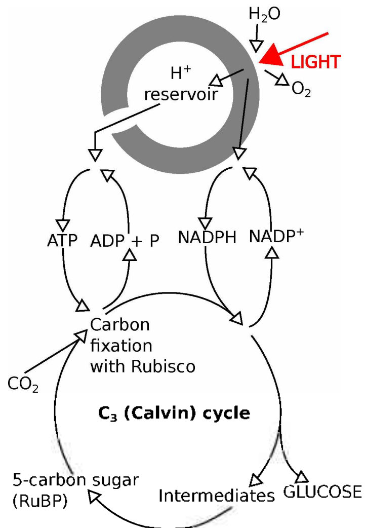
Figure 2.8. Summary of the photosynthesis. (Based on the idea from Arms & Camp, 1986).
