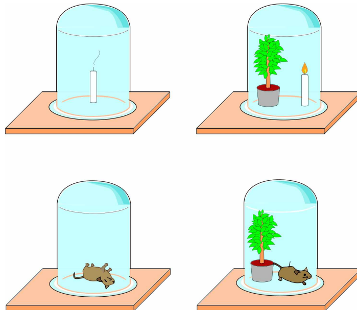
Figure 2.1. Experiments of J. Priestley (1772).
