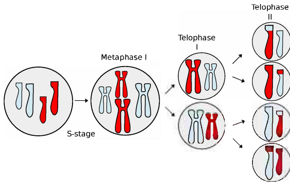
Figure 4.5. Principal scheme of meiosis. Only one of two telophase I variants is shown.
