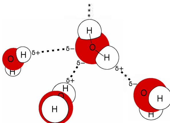
Figure 1.5. Hydrogen bonds between water molecules, \delta shows the partial charge.
