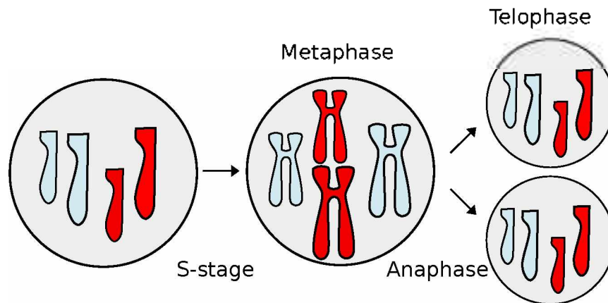
Figure 4.2. Principal scheme of mitosis.
