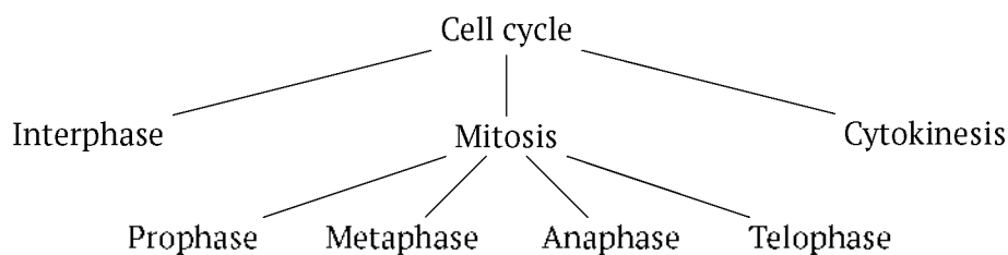
Figure 4.2. Principal scheme of mitosis.
