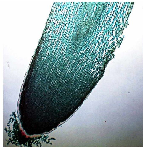
Figure 5.33. Left to right, top to bottom: Ranunculus root with 4-rayed xylem, Salix root with the lateral root developing, Smilax root with visible Casparian stripes in the endodermis; Zea root longitudinal section with root cap, division and elongation zones. Magnifications \times 100 (second) and \times 40 (others).
