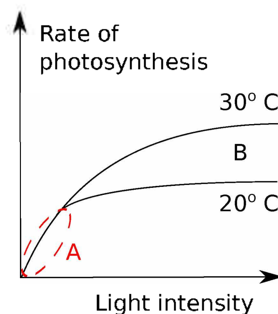
Figure 2.3. Explanation of experiment of F. Blackman (1905). A—low light, little temperature effect; B—high light, significant temperature effect.
