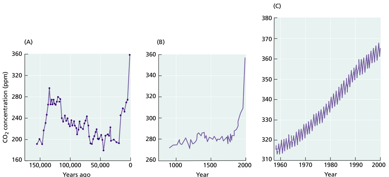
FIGURE 9.16 Concentration of atmospheric \text{CO}_2 from the present to 160,000 years ago. (A) Past atmospheric \text{CO}_2 concentrations, determined from bubbles trapped in glacial ice in Antarctica, were much lower than current levels. (B) In the last 1000 years, the rise in \text{CO}_2 concentration coincides with the Industrial Revolution and the increased burning of fossil fuels. (C) Current atmospheric concentrations of \text{CO}_2 measured at Mauna Loa, Hawaii, continue to rise. The wavy
