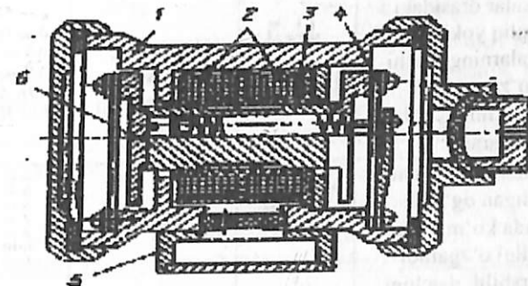
12.2 - rasm. Vibratsion siljishlar datchigi
