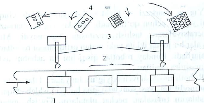
7.1 - rasm. Detaillar magazinidan foydalanish sxemaşi:
