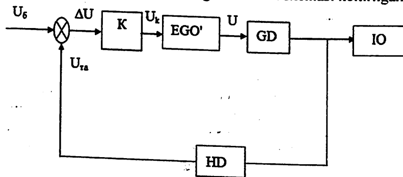
3.3 – rasm. Sanoat roboti elektrogidravlik yuritmasining funksional sxemasi:
