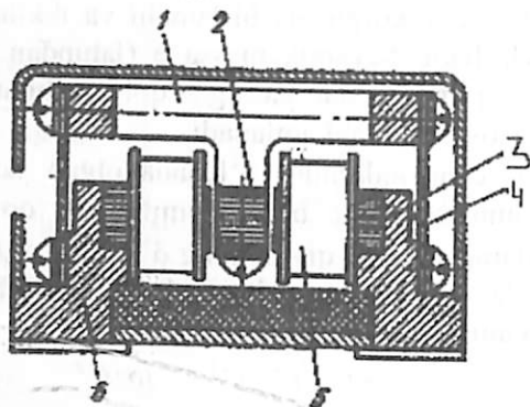
12.3 - rasm. Tezlanishni o'lchash uchun datchik
