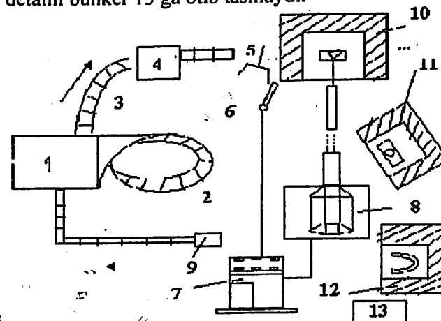
8.7 - rasm. Issiq shtamlash RTKsi:
