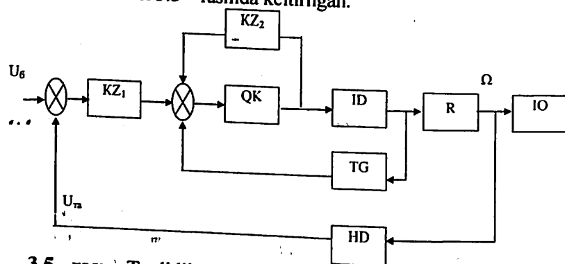
3.5 - rasm. Taqlidli elektrik yuritmaning funksional sxemasi:
