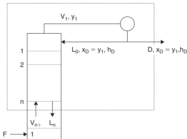
Figure 13.9 Material balance for the rectifying section
