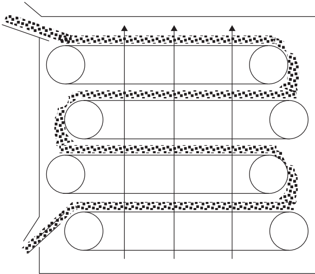
Figure 22.19 Multistage belt dryer
