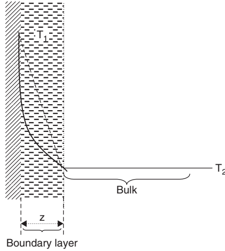
Figure 3.6 Boundary layer in turbulent convection
