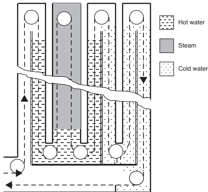
Figure 18.11 Hydrostatic sterilizer
