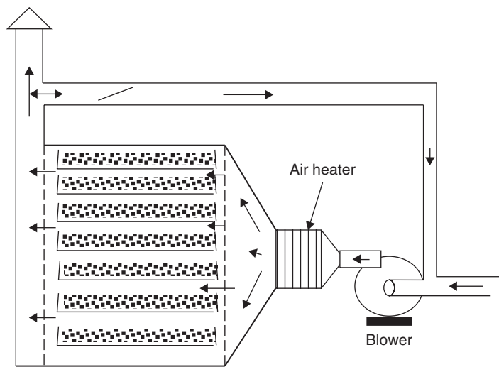
Figure 22.15 Cabinet dryer
