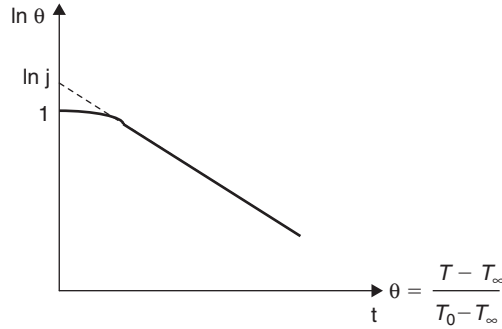
Figure 3.9 General form of unsteady state heat transfer plot
