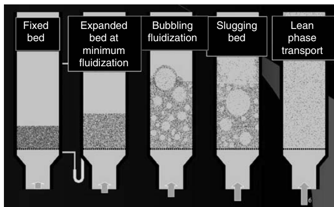
Figure 2.37 Stages of fluidization. (Courtesy of GEA-NIRO)
