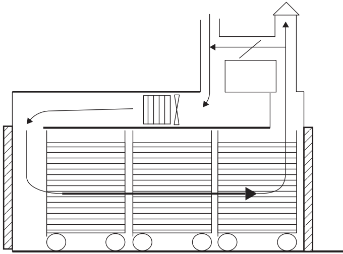
Figure 22.16 Short tunnel dryer
