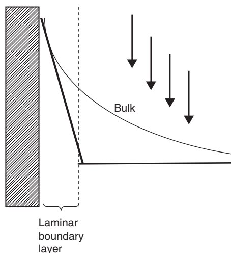
Figure 2.6 Boundary layer in turbulent flow
