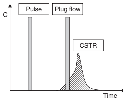
Figure 4.10 Reaction of plug-flow reactor and a CSTR to a pulse injection
