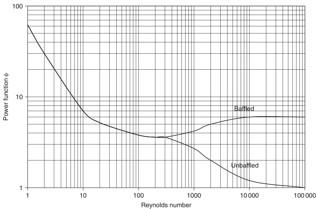
Figure A.3 Mixing power function, turbine impellers
