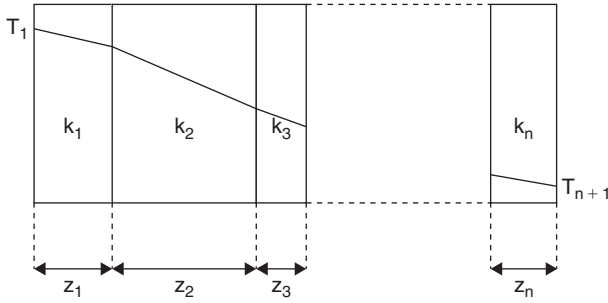
Figure 3.3 Conduction in multilayer slab
