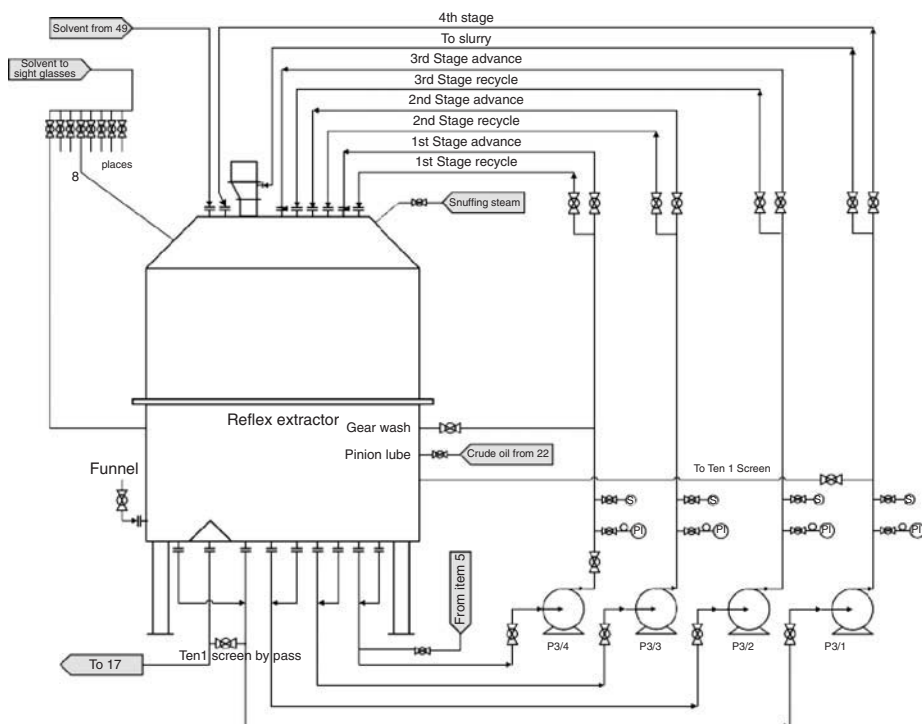
Figure 11.9 Carrousel extractor. (Courtesy of DeSmet-Balestra A.G.)
