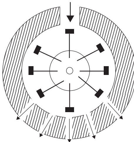
Figure 6.5 Basic structure of a hammer mill
