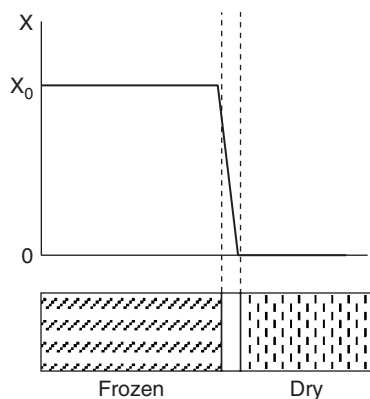
Figure 23.2 Moisture distribution in a material undergoing freeze drying
