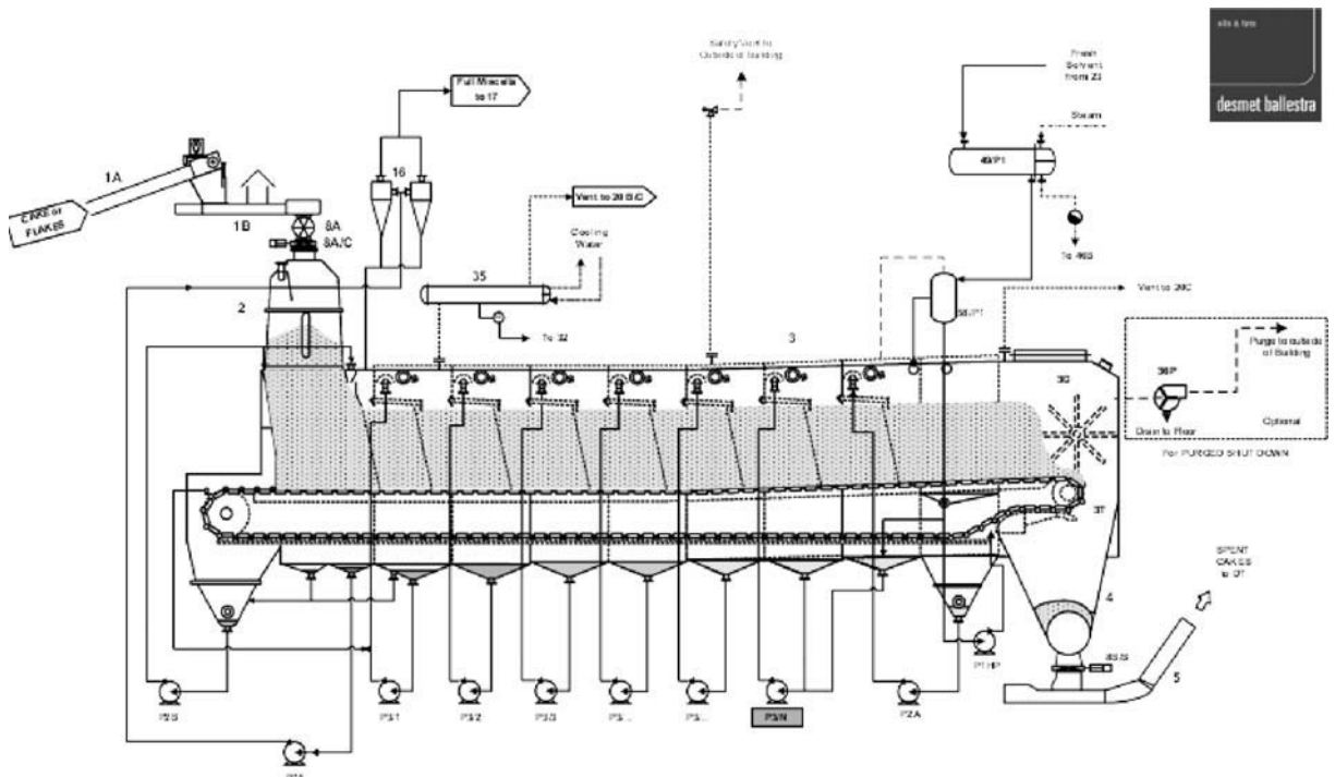
Figure 11.8 Belt extractor. (Courtesy of DeSmet-Ballestra A.G.)
