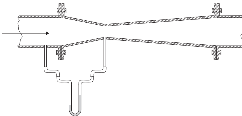
Figure 5.16 Venturi flow meter
