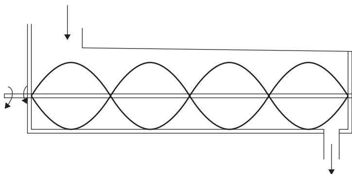
Figure 7.15 Ribbon mixer
