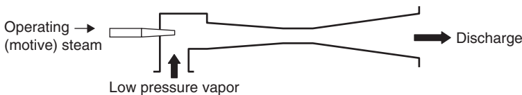
Figure 2.25 Steam-jet ejector
