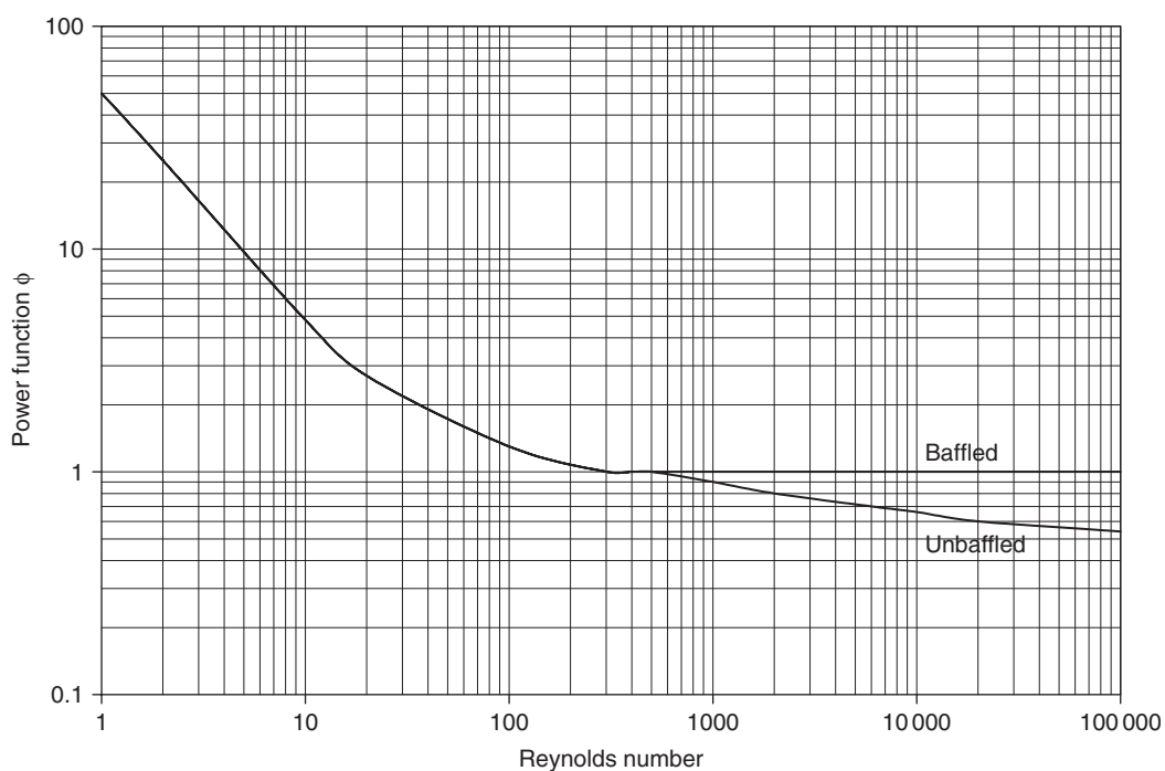
Figure A.4 Mixing power function, propeller impellers
