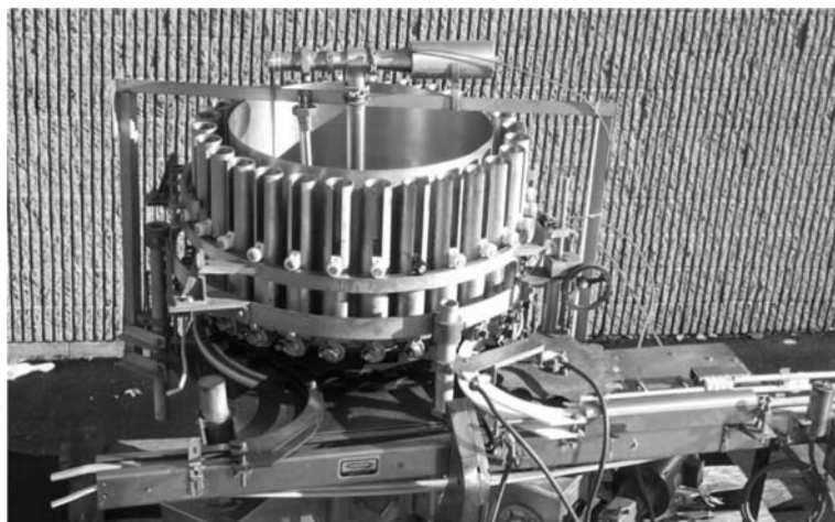
Figure 18.3 Piston filler
