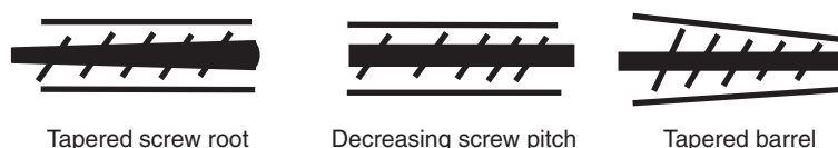
Figure 15.2 Three methods to achieve compression
