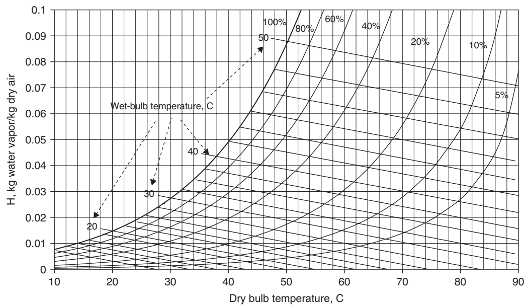
Figure A.2 Psychrometric chart
