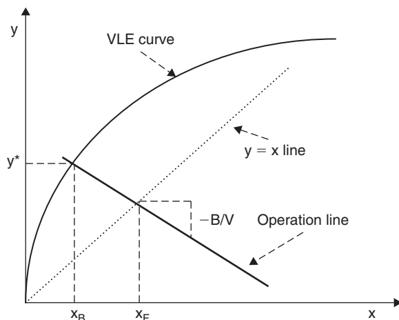
Figure 13.3 Graphical representation of flash distillation
