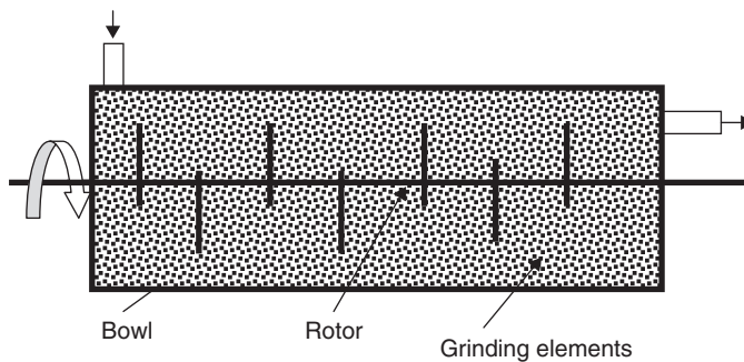
Figure 6.14 Wet ball-mill
