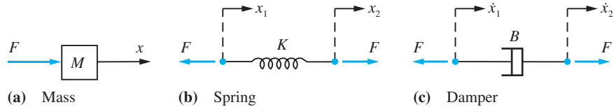
Figure 11.11 Constituent elements of a translational mechanical system.
