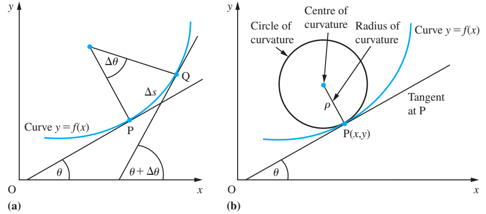
Figure 8.29 Curvature and radius of curvature.
