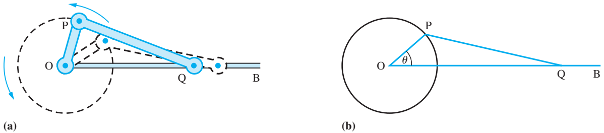
Figure 12.24 Slider–crank mechanism.
