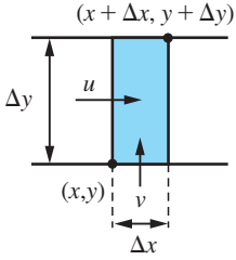
Figure 9.24 Flow through rectangular element.
