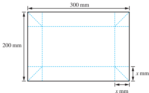
Figure 1.9 Sheet of cardboard of Question 19.
