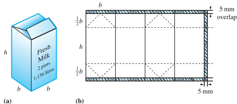
Figure 8.39 The construction of a milk carton.
