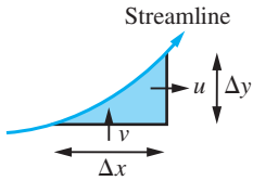
Figure 9.25 Streamline.
