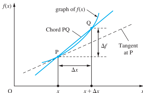
Figure 8.4 Illustration of derivative as slope of a tangent.
