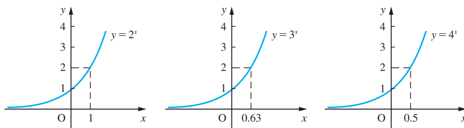
Figure 2.82 Scaled graphs of exponential functions.
