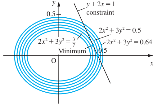
Figure 9.21 Level curves of f(x, y) = 2x^2 + 3y^2 .
