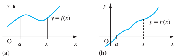
Figure 8.52 (a) Graph of y = f(x) . (b) Graph of \int_a^x f(t)dt .
