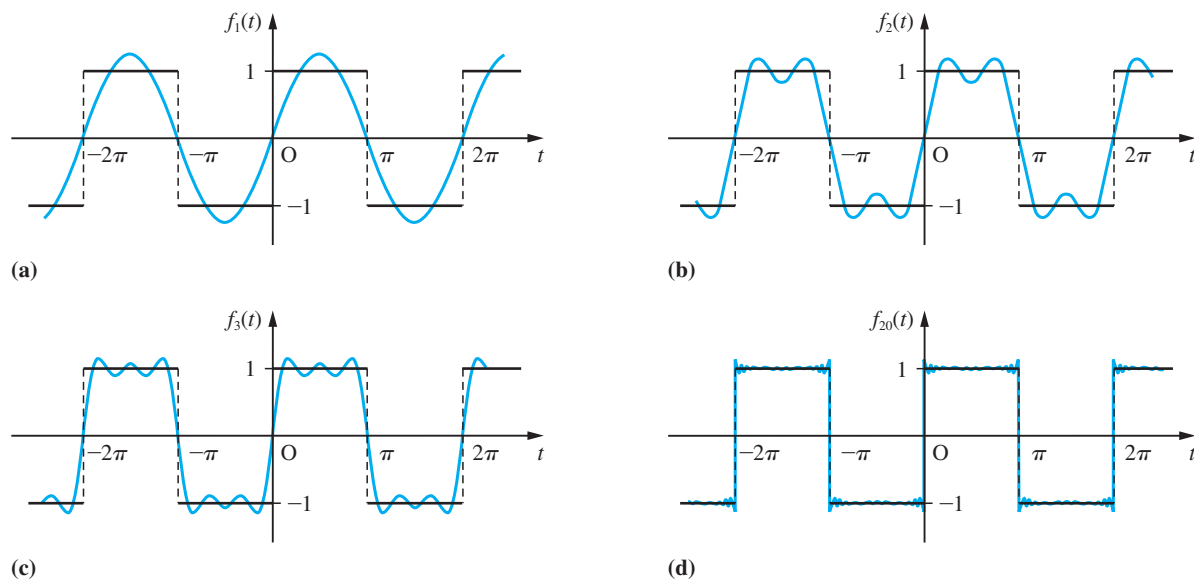
Figure 12.11 Plots of f_N(t) for a square wave: (a) N = 1 ; (b) 2; (c) 3; (d) 20.
