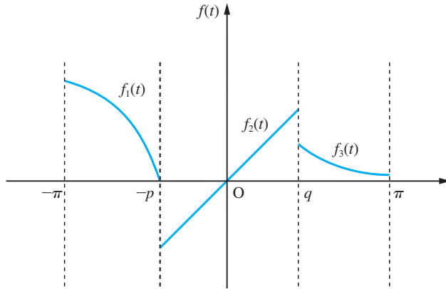
Figure 12.4 Piecewise-continuous function over a period.
