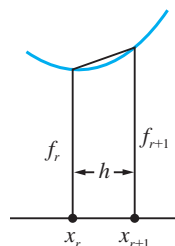
Figure 8.74 Trapezium approximation to area of strip.
