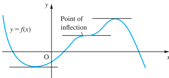
Figure 8.31 Graph with horizontal tangents.
