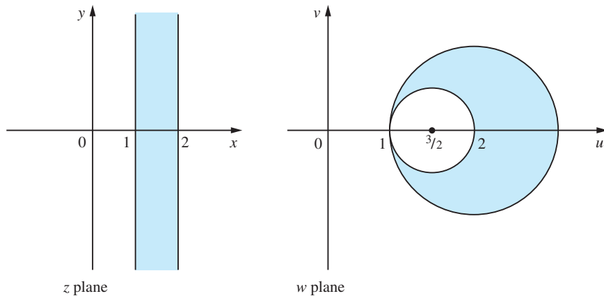
Figure 3.14 Transformation of the strip 1 < \operatorname{Re} z < 2 onto the w plane.
