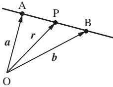
Figure 4.47 Line AB in terms of \vec{r} = \vec{OP} .
