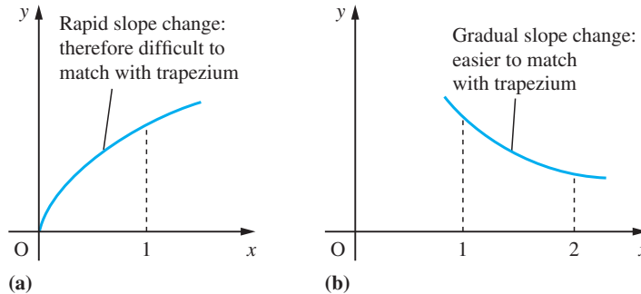
Figure 8.76 (a) Graph of y = \sqrt{x} . (b) Graph of y = 1/x .
