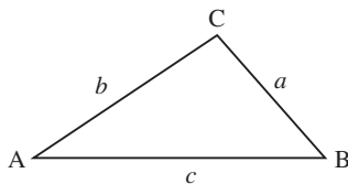
Figure 4.43 Sine rule: Section 2.6.1.
