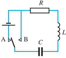
Figure 10.4 An inductor, capacitor, resistor ( LCR ) electrical circuit.
