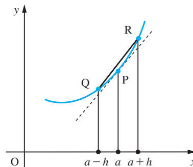
Figure 8.44 Chord approximation.
