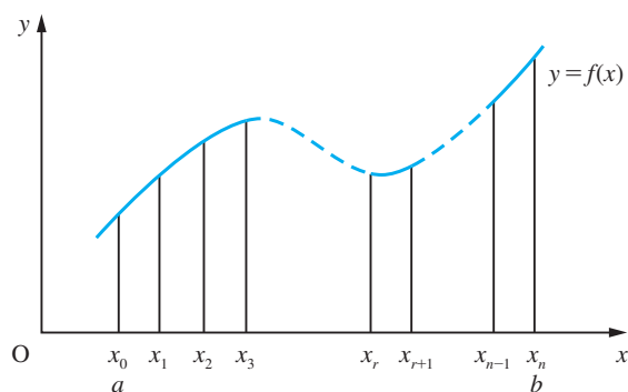
Figure 8.73 Slicing up an area into vertical strips of equal width.
