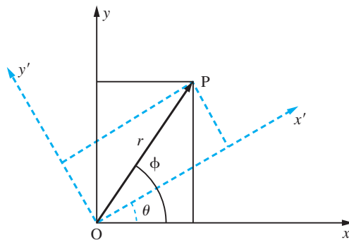
Figure 5.1 Change of axes from Oxy to Ox'y' .
