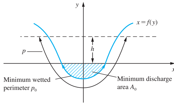
Figure 8.82 Channel cross-section.
