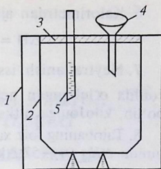
25-rasm. Kalorimetr: 1 — tashqi stakan; 2 — kalorimetrik stakan; 3 — qopqog'; 4 — voronka; 5 — termometr.
