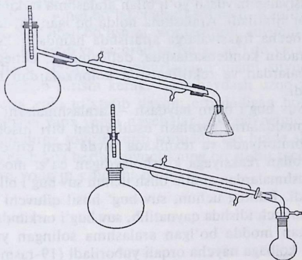
17-rasm. Oddiy sharoitda haydash.
