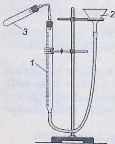
20-rasm. Ekvivalent aniqlanadigan asbob:
