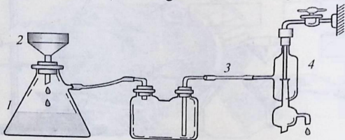
14-rasm. Past bosimda filtrlash.
