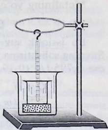
23-rasm. Soddalashtirilgan kalorimetr.
