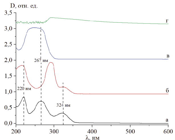
Fig. 1. Absorption spectra of the ternary chelate complex and the starting materials: а — absorption spectrum of iron ascorbatopyridoxine; б — absorption spectrum of pyridoxine; в — absorption spectrum of ascorbic acid; г — absorption spectrum of iron sulfate
