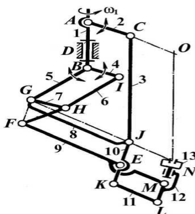
Fig. 2. Structural scheme of Osma manipulator pantograph
