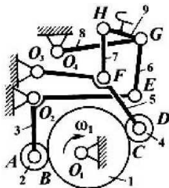
Fig. 1. Structural scheme of the knitting machine
