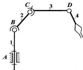
Fig. 3. Structural scheme of the spatial manipulator
