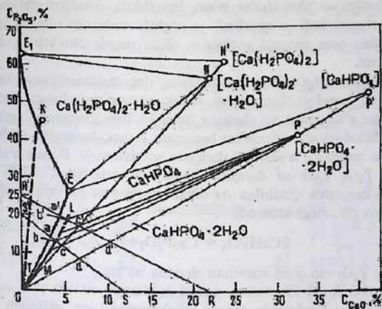
3.40-rasm. Fosfat kislotadan dikalsiy-fosfatni cho'ktirish jarayonining diagrammasi: 40°C dagi \text{CaO} - \text{P}_2\text{O}_5 - \text{H}_2\text{O} sistemasi izotemasida OE – stabil va ML – metastabil tarmog'i; 60°C dagi \text{CaO} - \text{P}_2\text{O}_5 - \text{H}_2\text{SiF}_6 - \text{H}_2\text{O} sistemasida KT – \text{CaHPO}_4 ning eruvchanlik tarmog'i.
