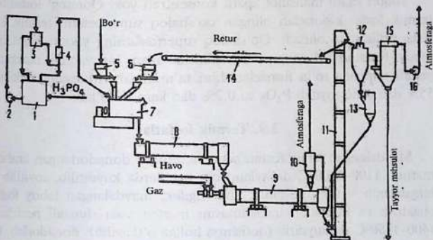
3.41-rasm. O'g'itli pretsipitat ishlab chiqarishning returli sxemasi: 1 – fosfat kislota yig'ichi; 2 – nasos; 3 – bak; 4 – sarflagich; 5,6 – bo'r va retur uchun bunkerlar; 7 – aralashtirgich; 8 – barabanli reaktor; 9 – barabanli quritgich; 10 – siklon; 11 – elevator; 12 – havoli separator; 13 – separatsiyalangan mahsulot yig'ichi; 14 – retur transportyori; 15 – yengli filtr; 16 – ventilator.
