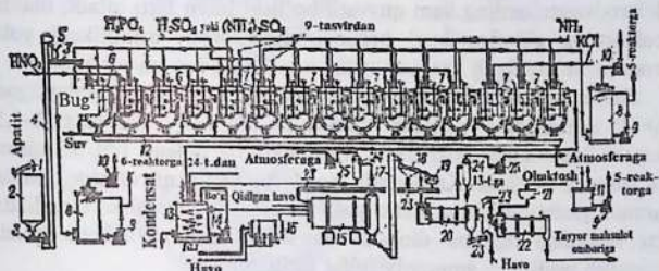
6.16-rasm. Nitrofoska ishlab chiqarish sxemasi: 1,23 – lentali konveyer; 2 – bunker; 3 – shnek; 4 – elevator; 5 – o'lchov me'yori; 6 – parchalanish uchun reaktorlar; 7 – ammoniyashtirish uchun reaktorlar; 8 – skruyer; 9 – markazdan qochma nasoslar; 10,25 – ventilatorlar; 11 – yig'gich; 12 – tarmov; 13 – suspenziya uchun yig'gich; 14 – suspenziya uchun nasos; 15 – BDG' jihozi; 16 – yondirgich; 17 – elevator; 18 – elak; 19 – tegirmon; 20 – sovitish barabani; 21 – qo'shimchani changlatish uchun bunker; 22 – konditsionirlash uchun baraban; 24 – siklonlar.
