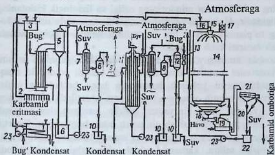
2.22-rasm. Donadorlangan karbamid olish tasviri: 1 – karbamid eritmasi uchun idish (yig'gich); 2 – press-filtr; 3,16 – baklar; 4 – birinchi bosqich bug'latish jihozining isitish kamerasi; 5 – separator; 6 – bug'langan eritma yig'gichi; 7 – yuza kondensatori; 8 – tomchi tutgich; 9 – vakuum-nasos; 10 – barometrik bak; 11 – ikkinchi bosqich rotor bug'latish jihozi; 12 – barometrik kondensator; 13 – bug' oqimli ektor; 14 – donadorlash minorasi; 15 – donadorlagich; 17 – ventilator; 18 – lentali transportyor; 19 – donachalarni «qaynovchi qatlam» da sovitgich; 20 – elevator; 22 – chang va yirik donachalarni eritish baki; 23 – markazdan qochma nasos.
