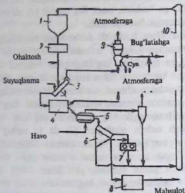
2.12-rasm. «Norsk-Hydro» («Norsk-Gidro») firmasi usuli bo'yicha tarekali donadorlagichdan foydalanib, donadorlangan ammiakli va ohakli-ammiakli selitralar olishning texnologik sxemasi: 1 – retur bunker; 2 – ta'minlagich; 3–tarekali donadorlagich; 4 – shliflovchi baraban; 5 – sovitgich; 6 – clak; 7 – tegirmon; 8 – kukunlashtiruvchi barabanlar; 9 – skruber; 10 – elevator.
