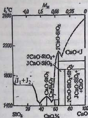
3.10-rasm. CaO – SiO 2 sistemasining holat diagrammasi.
