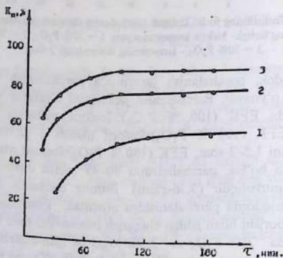
3.36-rasm. Fosforitning fosfat kislotali parchalanish darajasining vaqt bo'yicha o'zgarishi: -kislota konsentratsiyasi: 1-37% P_2O_5 ; 2-35% P_2O_5 ; 3-30% P_2O_5 ; - EFK( 100\% P_2O_5 ):fosforit nisbat: 1-1:1; 2-1,5:1; 3-1,5:1; - jarayonning harorati: 1-60°C; 2-60°C; 3-80°C.
