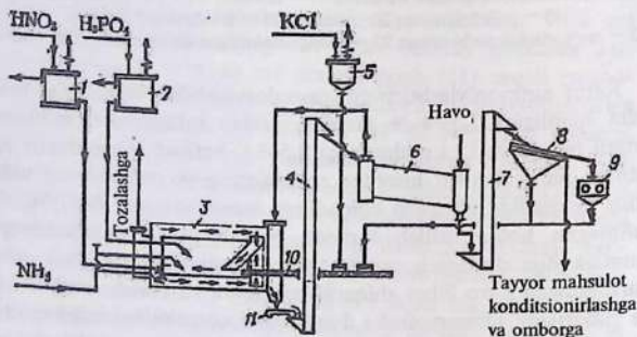
6.15-rasm. Murakkab o'g'it ishlab chiqarishning kam returli sxemasi: 1 – HNO_3 uchun quyuvshi bak; 2 – H_3PO_4 uchun quyuvshi bak; 3 – ammoniy lashtiruvchi donadorlagich; 4 – elevator; 5 – KCl uchun bunker; 6 – sovitish barabani; 7 – elevator; 8 – elak; 9 – tegirmon; 10 – shnek; 11 – lentali konveyer.
