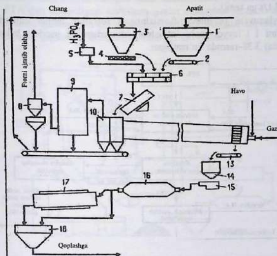
3.37-rasm. Aylanuvchi pechlarda ftorsizlangan fosfatlar ishlab chiqarish sxemasi: 1 – apatit uchun bunker; 2 – og'irlik o'lchov me'yoralashtirgichi; 3 – chang uchun bunker; 4 – ta'minlagich; 5 – fosfat kislota me'yoralashtirgichi; 6 – ikki valli aralashtirgich; 7 – likopchasimon donadorlagich; 8 – siklon (chang tutgich); 9 – issiqlik yutdirish qozoni; 10 – changli kamera; 11 – aylanuvchi pech; 12 – rekuperator; 13 – konveyer; 14 – klinker (qorishma) uchun bunker; 15 – tebranuvchi ta'minlagich; 16 – tegirmon; 17 – sovitish barabani; 18 – tayyor mahsulot saqlanadigan bunker.
