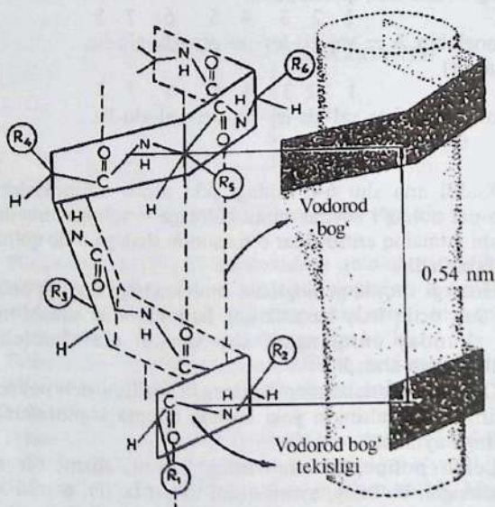
5-rasm. Peptid zanjirining \alpha -spirali.
