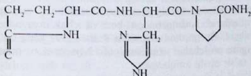
Piroglutamil-gistidil-prolinamid
