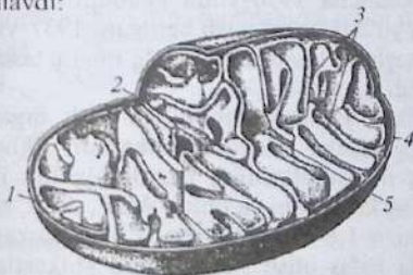
13-rasm. Mitoxondriyaning tuzilishi:
