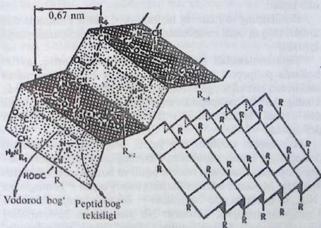
6-rasm. Peptid zanjirining \beta -tuzilishi.
