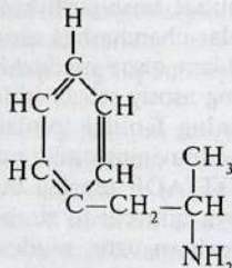
Fenamin
